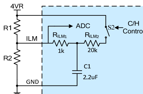
Figure 16. ILM vs. Cooling and Heating Control
