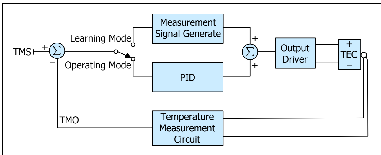
Figure 7. Auto PID System Block Diagram
