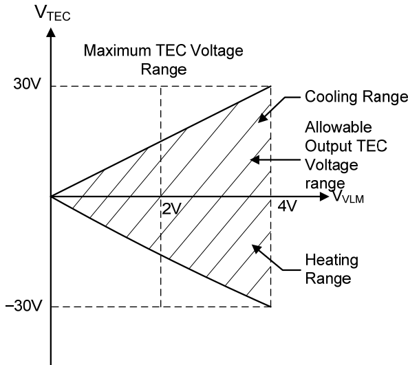
Figure 17. V TEC vs. V LM
