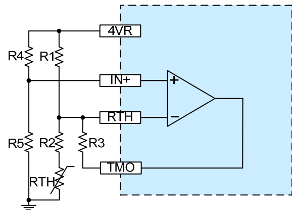
Figure 9.2. RTH
