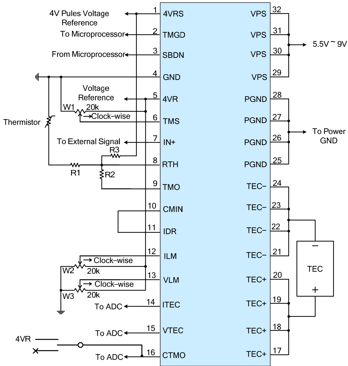
Figure 8.2. Connection for TEC9V6ADAPID & TEC9V6ASAPID
