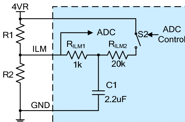
Figure 15. ILM vs. Cooling and Heating Control The switch S1 is closed @ heating, and open @ cooling
