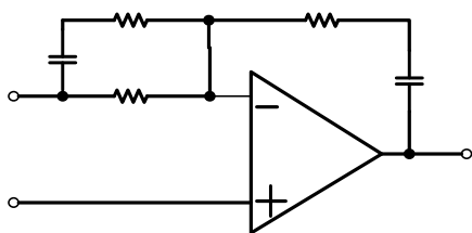
Figure 26. Compensation Network
