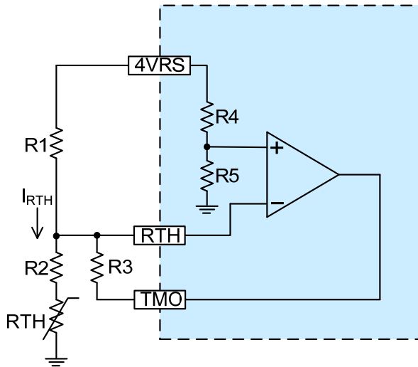
Figure 8. Thermistor
