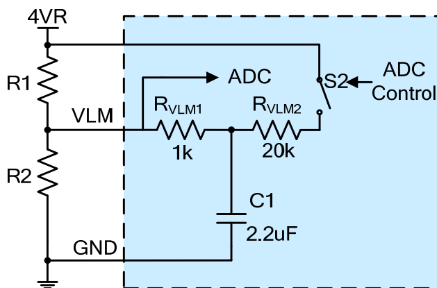
Figure 17. VLM vs. Cooling and Heating Control
