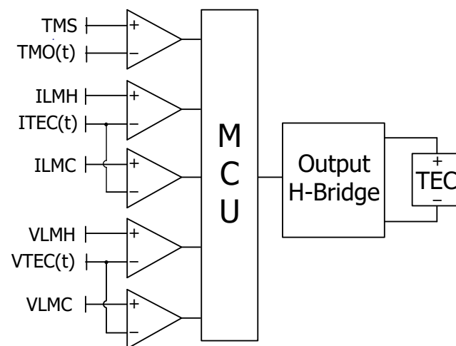
Figure 7. Key Control Loops of TEC24V6A
