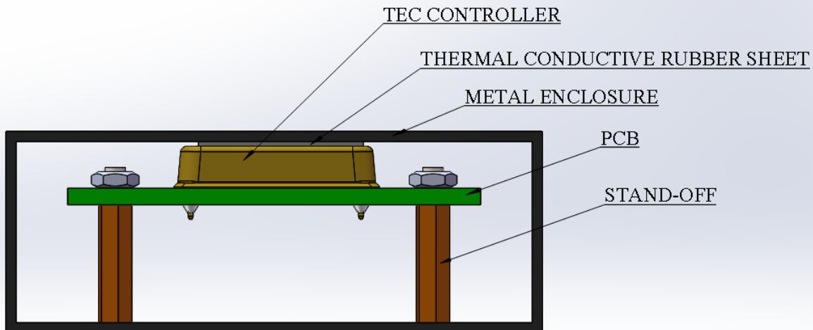
Figure 37. Transferring Heat with Metal Enclosure
