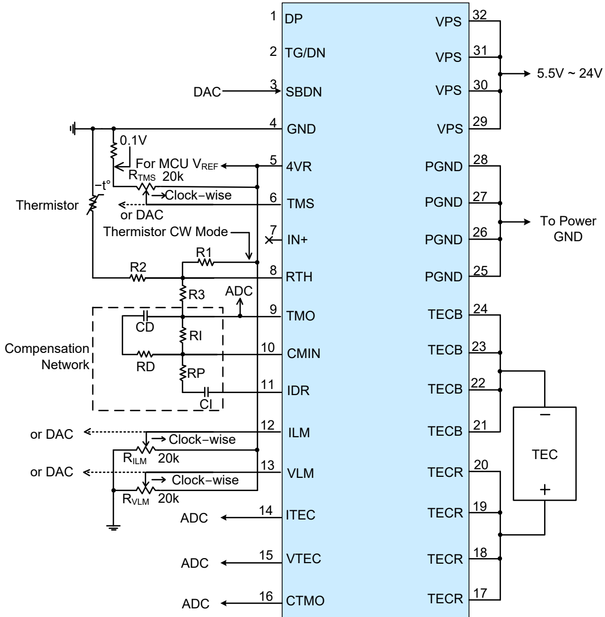
Figure 11.1. Using External Analog Compensation Network
