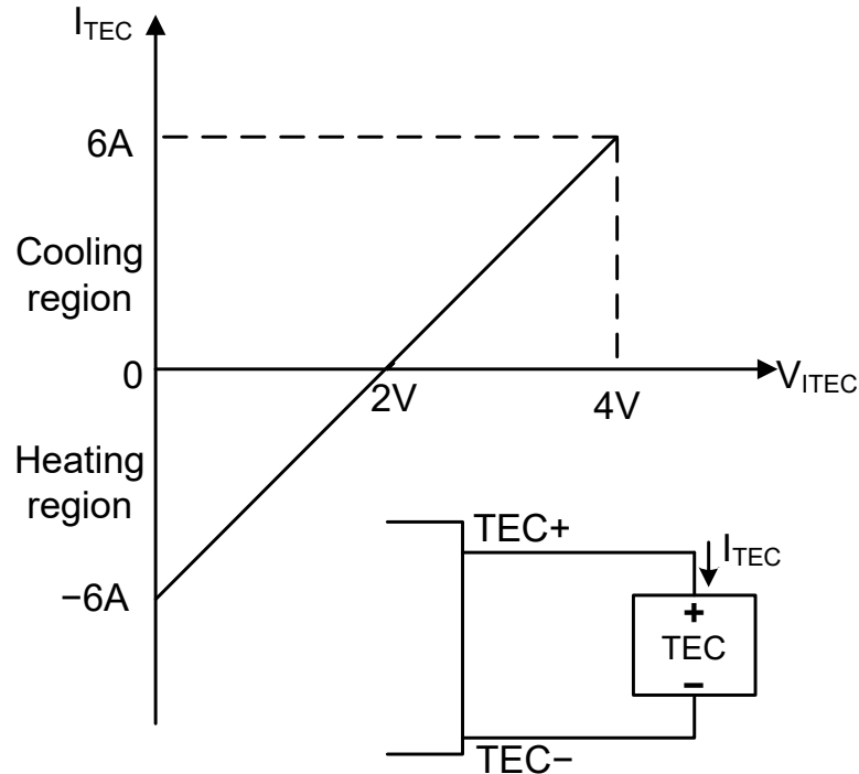
Figure 19. V_{ITEC} vs. I_{TEC}
