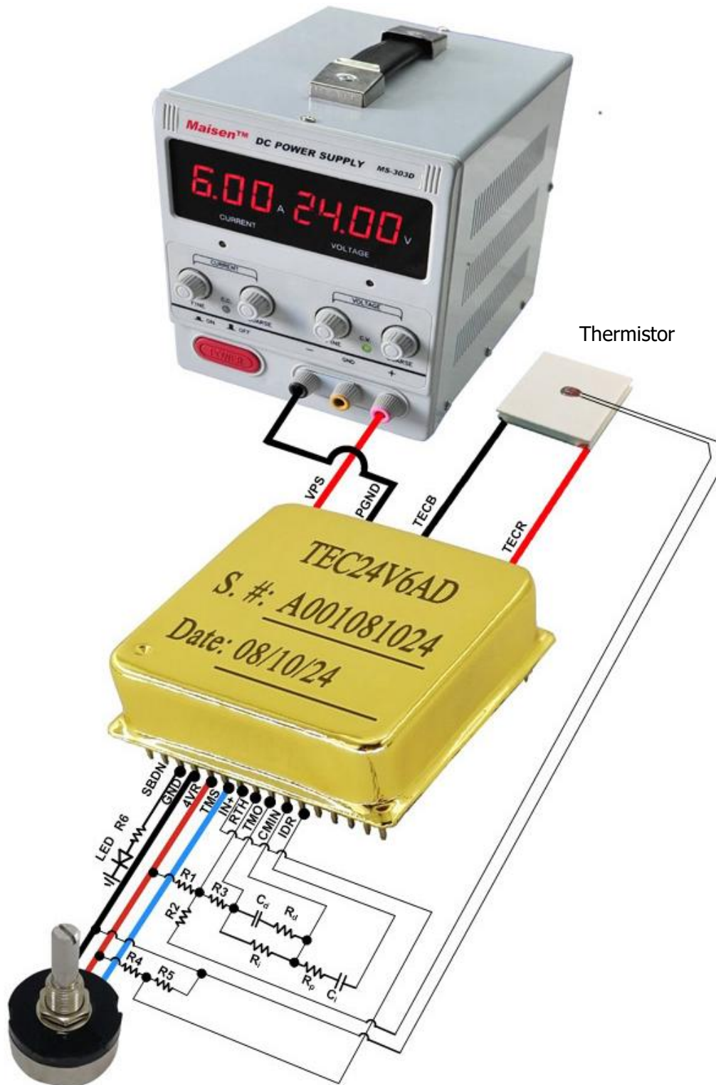
Figure 3. A 3-D Schematic Drawing for Using TEC24V6AD TEC Controller
