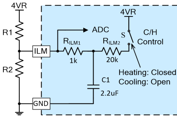
Figure 21. ILM vs. Cooling and Heating Control
