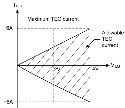
Figure 20. V_{ILM} vs. I_{TEC}
