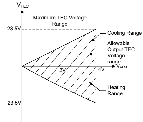
Figure 22. V_{TEC} vs. V_{LM}
