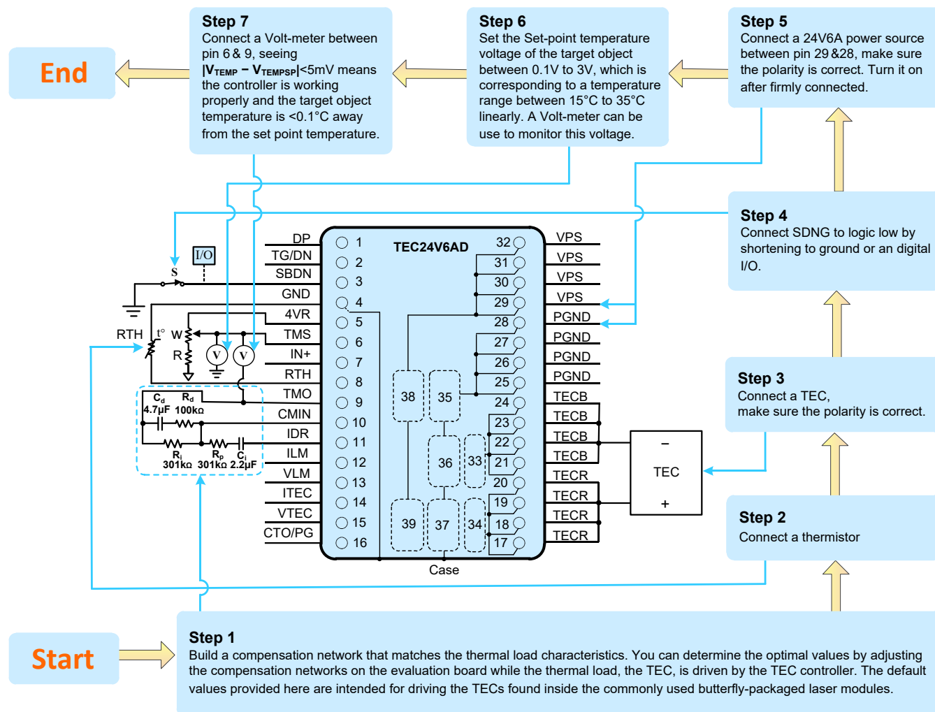
Figure 4. Operation Steps
