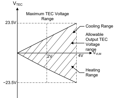
Figure 22. V_{TEC} vs. V_{VLM}
