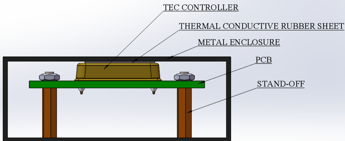
Figure 37. Transferring Heat with Metal Enclosure
