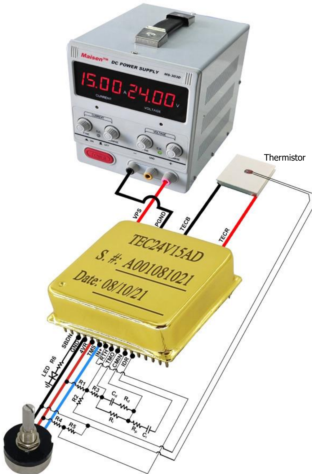
Figure 3. A 3-D Schematic Drawing for Using TEC24V15AD TEC Controller
