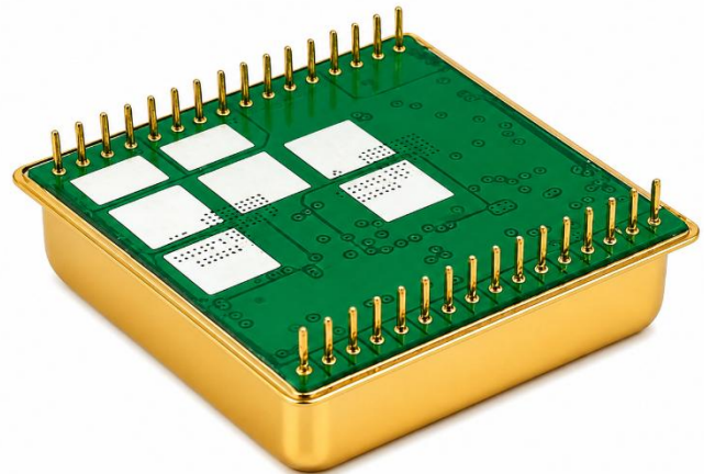
Figure 2. Bottom View of TEC24V15AD
