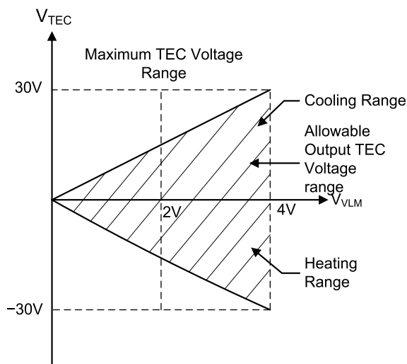
Figure 17. V_{TEC} vs. V_{LM}
