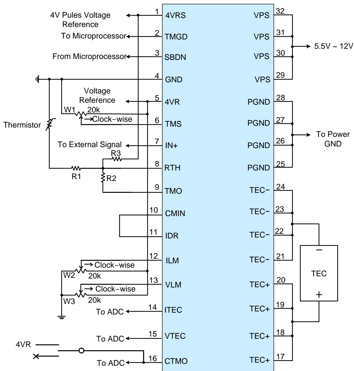
Figure 8.2. Connection for TEC12V9ADAPID & TEC12V9ASAPID
