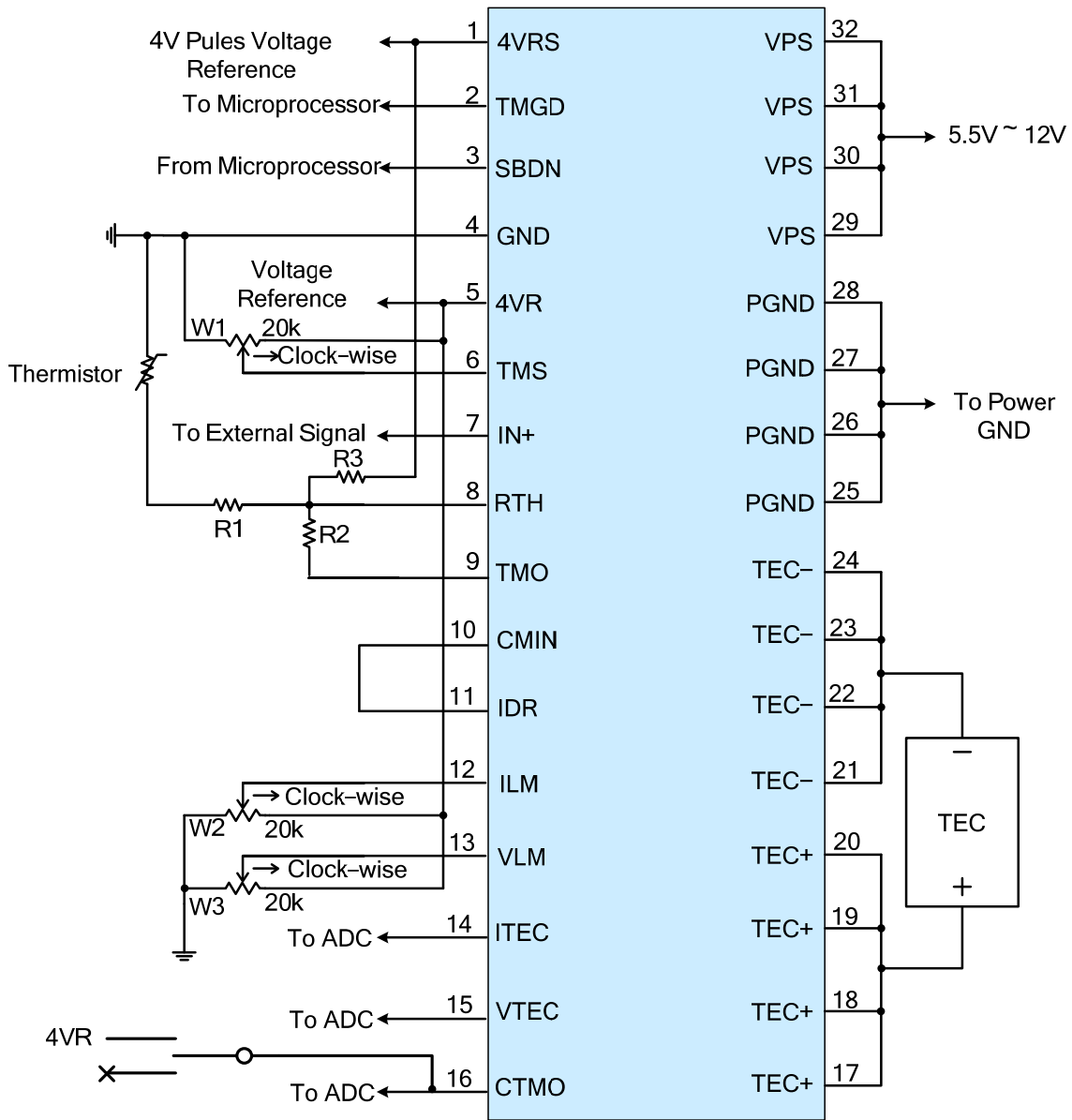
Figure 8.2. Connection for TEC12V6ADAPID & TEC12V6ASAPID
