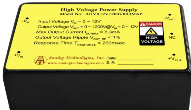
Figure 1. Physical Photos of AHVR12V1200V8R3MAP
