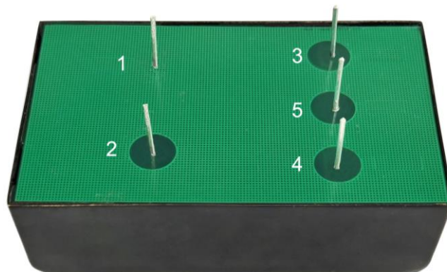
Figure 1. Physical Photos of AHVR12V1200V8R3MAP
