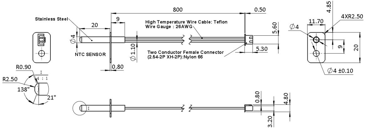
Figure 2. Component outline of the ATSC230K-100
