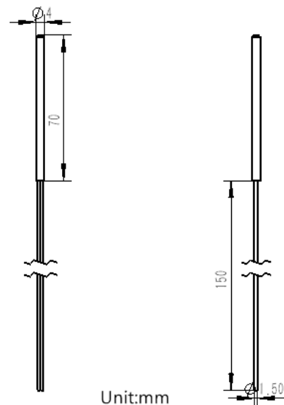
Figure 2. The Front and Side Views of ATSC10KF1-S6
