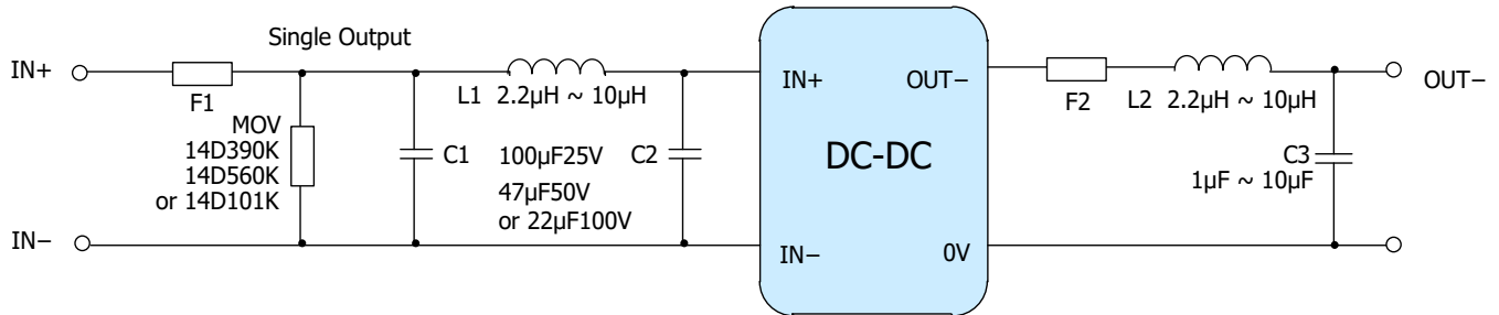
Figure 6. Typical Applications
