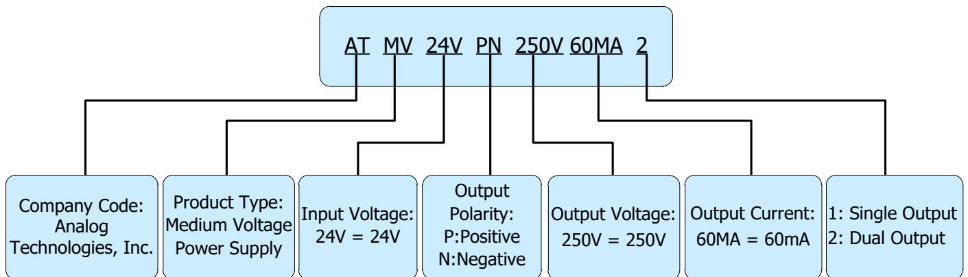
Figure 9. Naming Convention of ATMV24VPN250V60MA2
