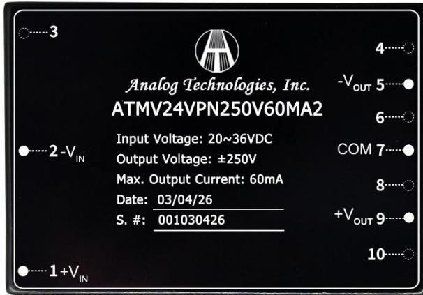
Figure 5. Top View
