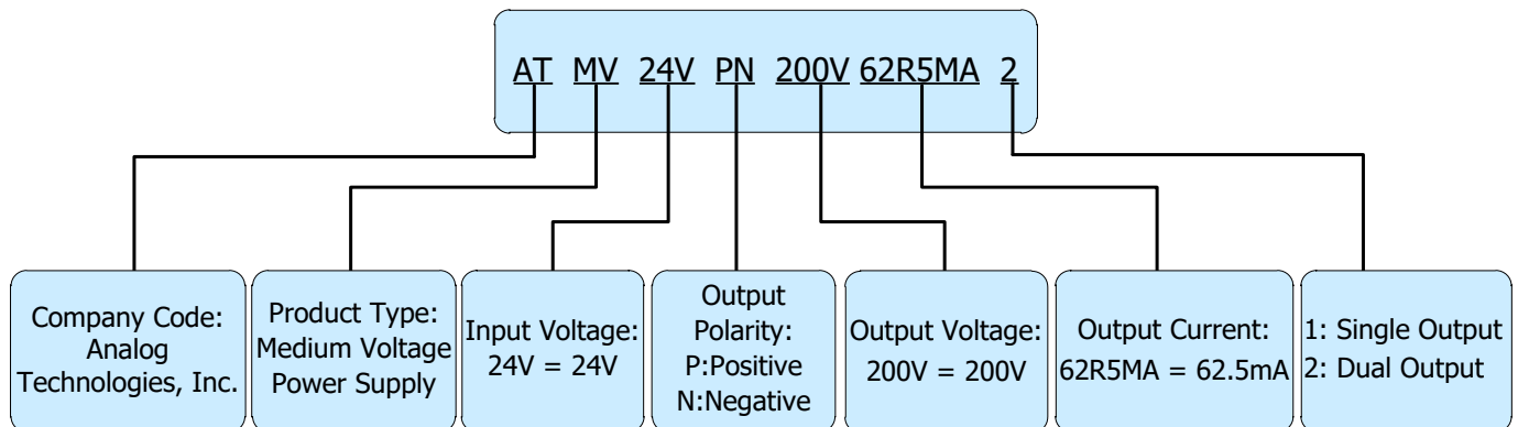
Figure 9. Naming Convention of ATMV24VPN200V62R5MA2
