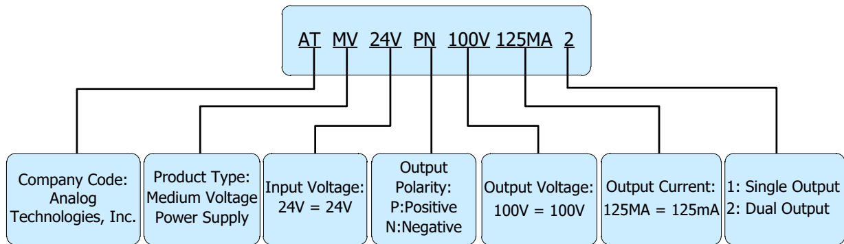
Figure 9. Naming Convention of ATMV24VPN100V125MA2
