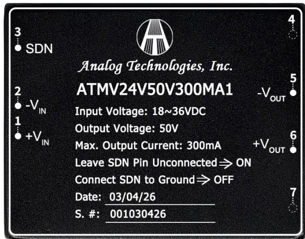
Figure 5. Top View
