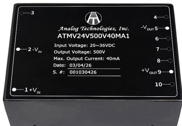
Figure 1. Top View ATMV24V500V40MA1
