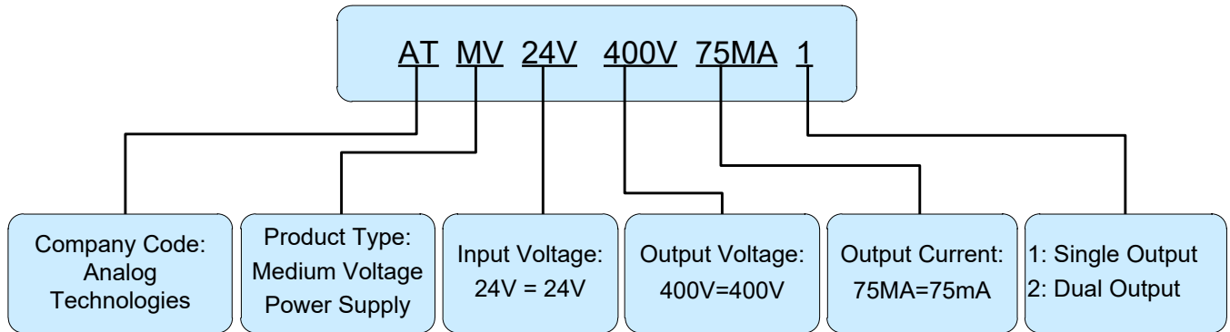
Figure 9. Naming Convention of ATMV24V400V75MA1
