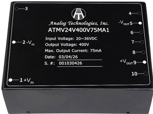
Figure 1. Top View ATMV24V400V75MA1
