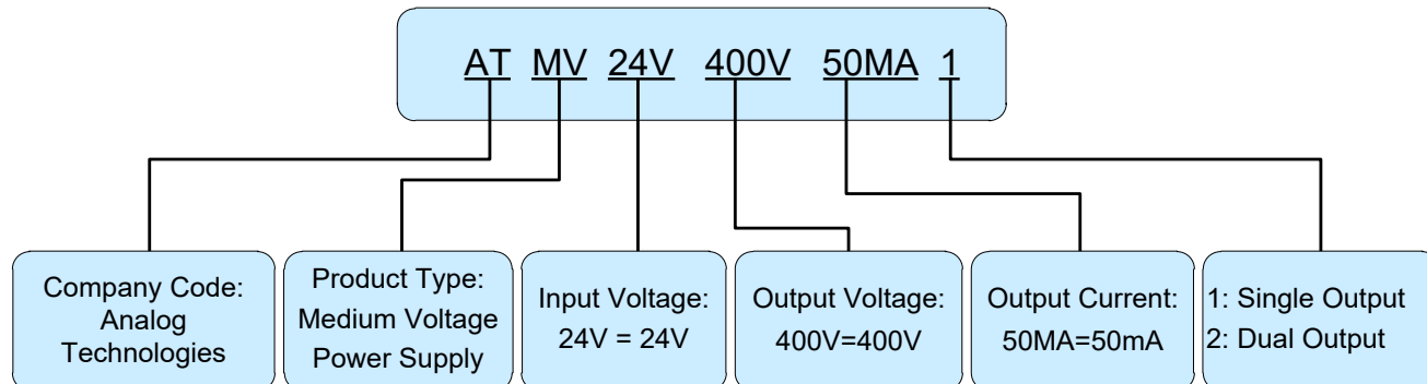
Figure 9. Naming Convention of ATMV24V400V50MA1
