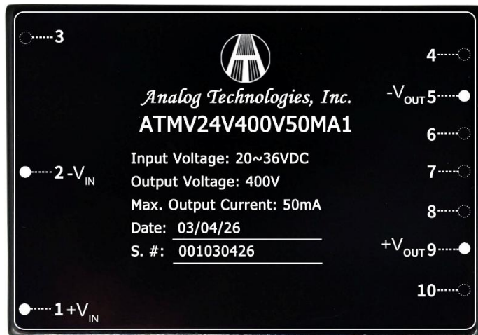
Figure 5. Top View
