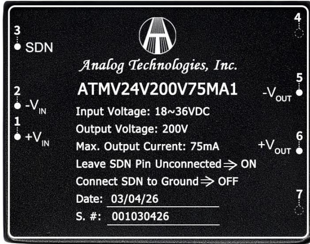
Figure 5. Top View
