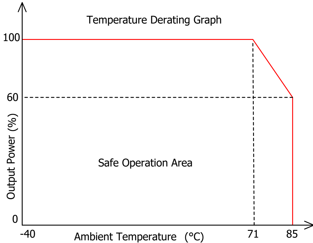
Figure 7. Derating Curve
