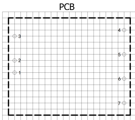
Figure 10. Outline Dimensions
