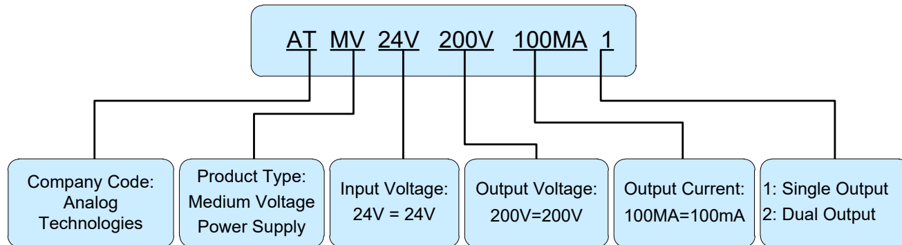
Figure 9. Naming Convention of ATMV24V200V100MA1
