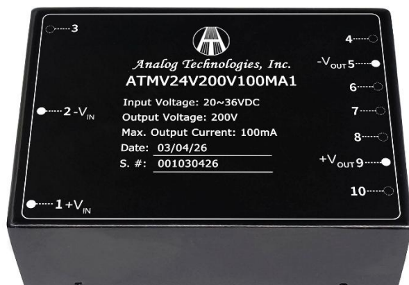
Figure 1. Top View ATMV24V200V100MA1
