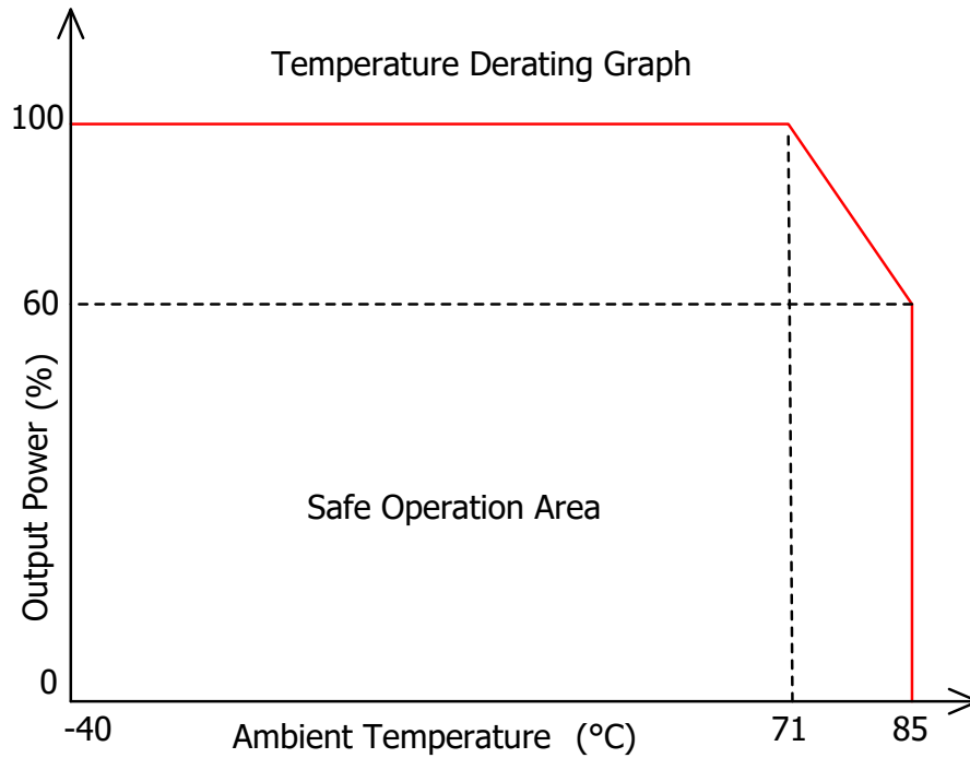
Figure 7. Derating Curve
