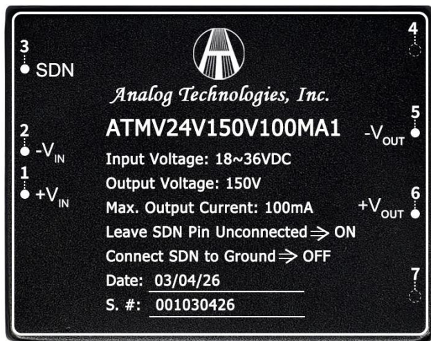
Figure 5. Top View
