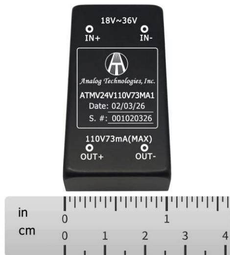
Figure 1. Top View
