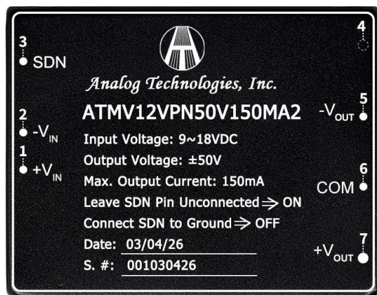
Figure 5. Top View
