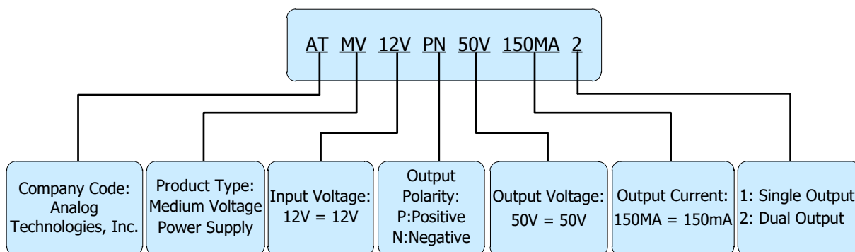
Figure 9. Naming Principle of ATMV12VPN50V150MA2
