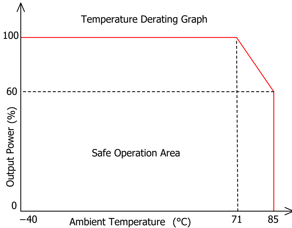
Figure 7. Derating Curve
