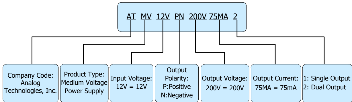
Figure 9. Naming Convention of ATMV12VPN200V75MA2
