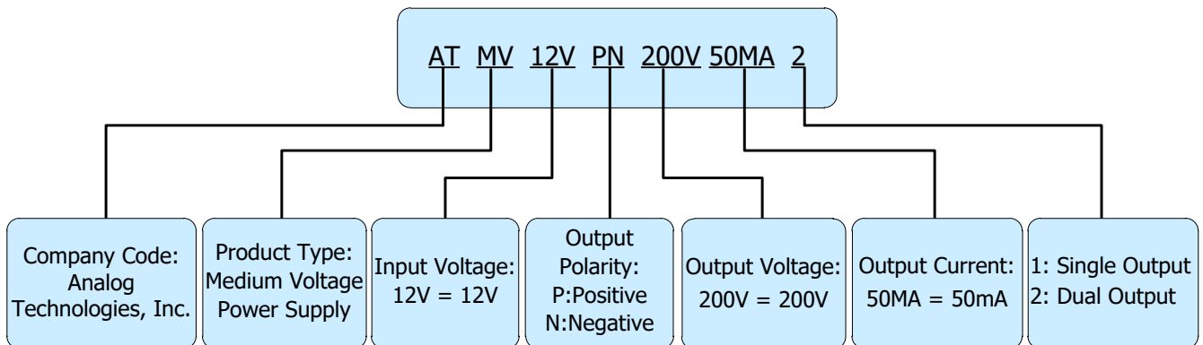
Figure 9. Naming Convention of ATMV12VPN200V50MA2
