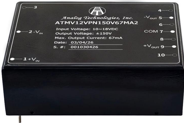
Figure 1. Top View ATMV12VPN150V67MA2
