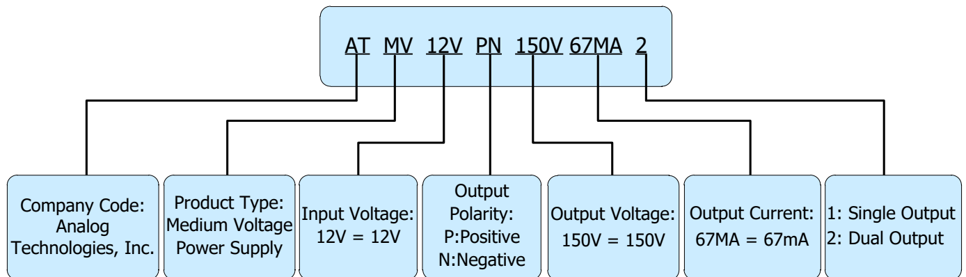
Figure 9. Naming Convention of ATMV12VPN150V67MA2
