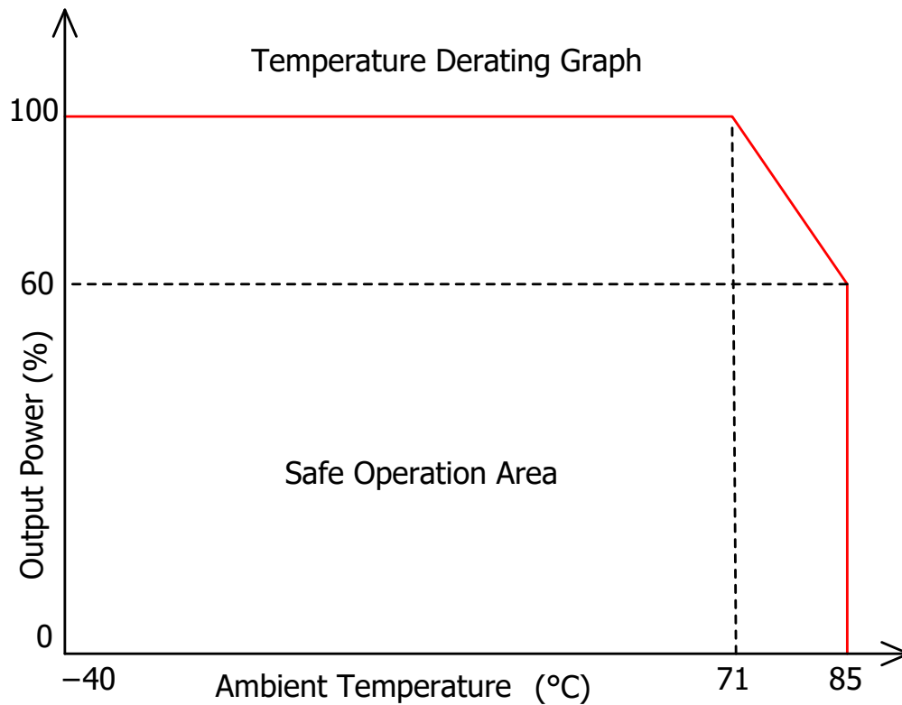
Figure 7. Derating Curve
