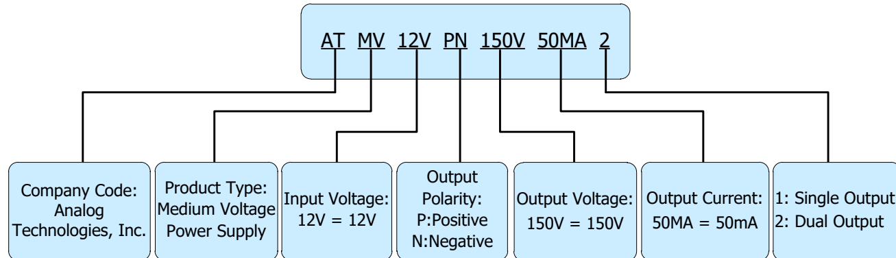
Figure 9. Naming Principle of ATMV12VPN150V50MA2
