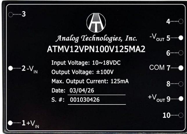
Figure 5. Top View
