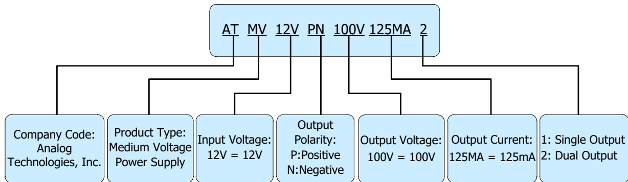
Figure 9. Naming Convention of ATMV12VPN100V125MA2
