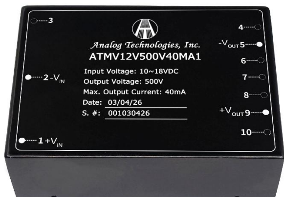
Figure 1. Top View ATMV12V500V40MA1
