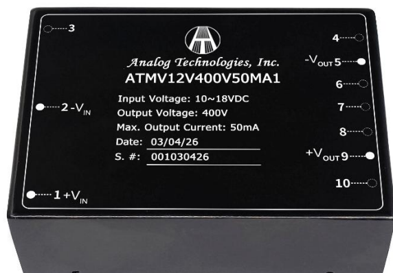
Figure 1. Top View ATMV12V400V50MA1
