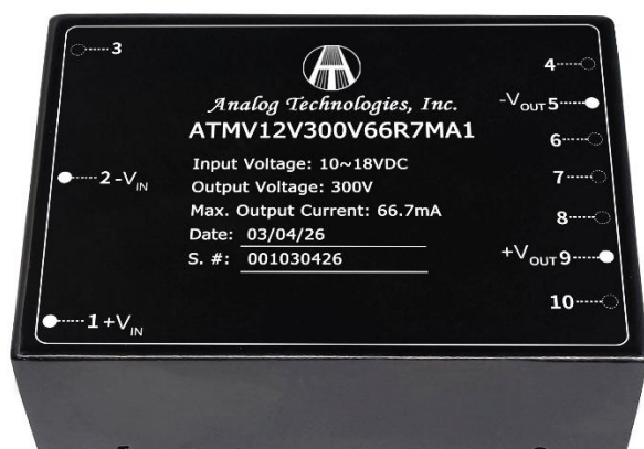
Figure 1. Top View ATMV12V300V66R7MA1
