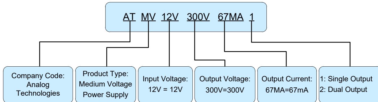
Figure 9. Naming Convention of ATMV12V300V67MA1
