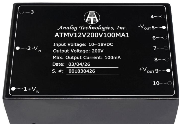
Figure 1. Top View ATMV12V200V100MA1
