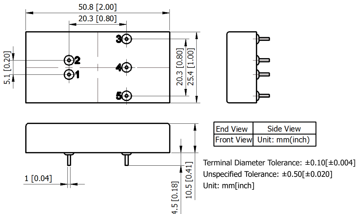
Figure 7. Outline Dimensions
