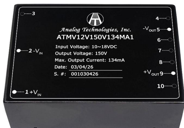
Figure 1. Top View ATMV12V150V134MA1
