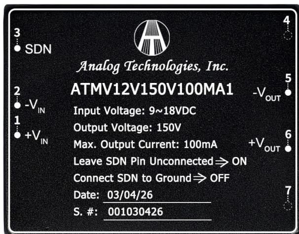
Figure 5. Top View
