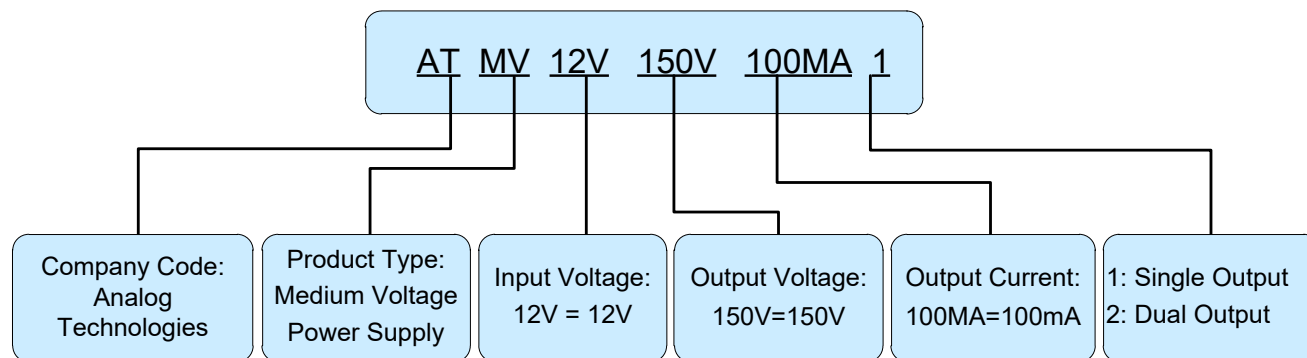
Figure 9. Naming Convention of ATMV12V150V100MA1
