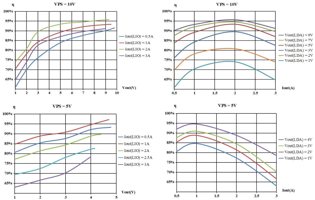
Figure 11. Efficiency of Laser Driver
