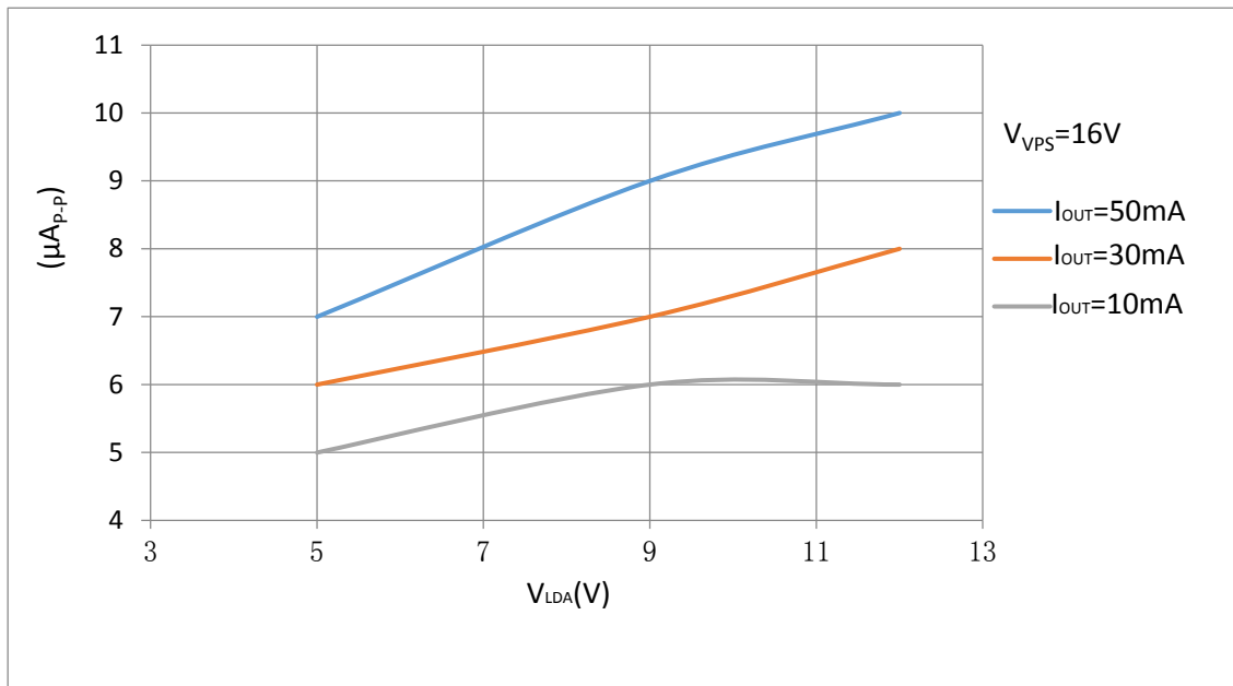
Figure 12.1. V_{LDA} vs. Output Current Noise@0.1Hz~10Hz
