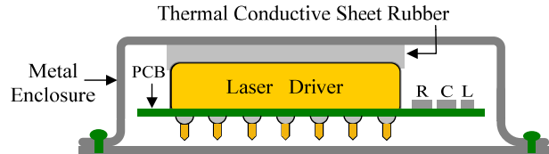
Figure 11. Transferring heat by the gap filler
