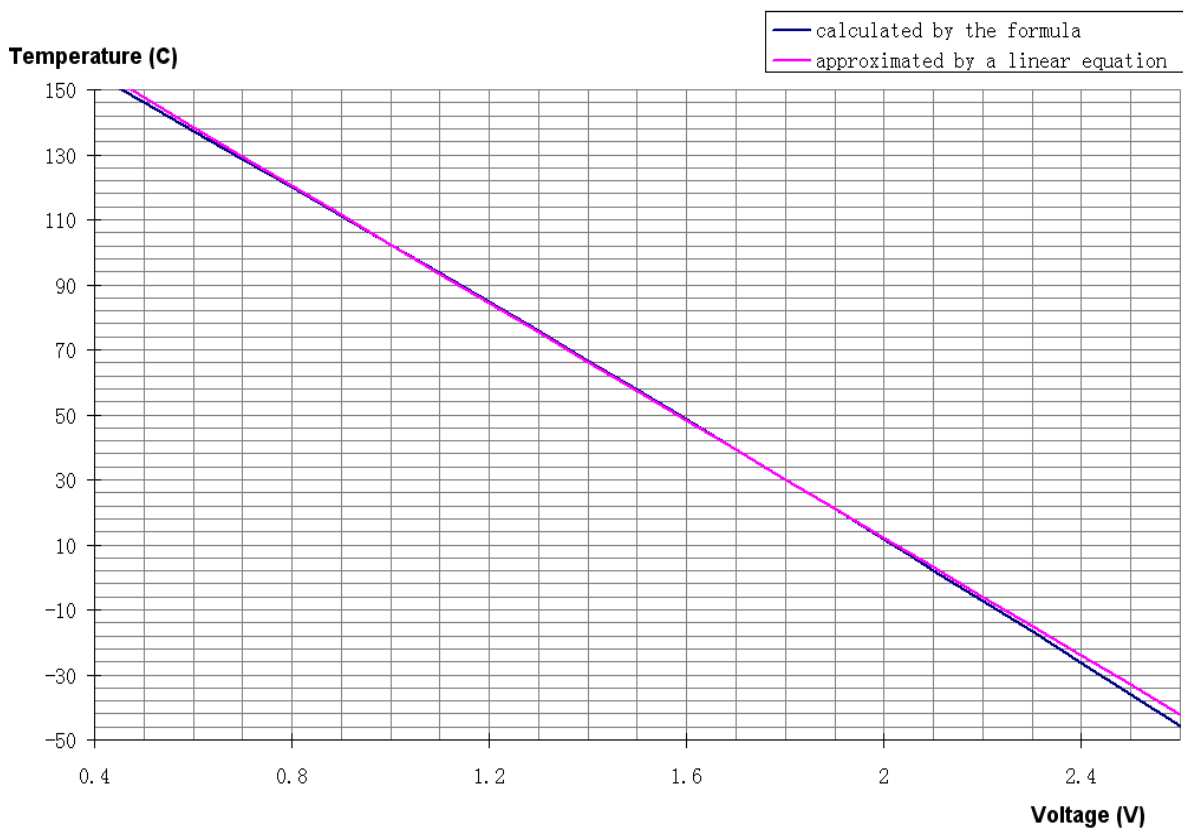
Figure 7. Controller Internal Temperature vs. TMPO Voltage
