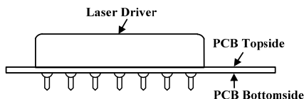
Figure 16. Side View of the Laser Driver mounted on PCB
