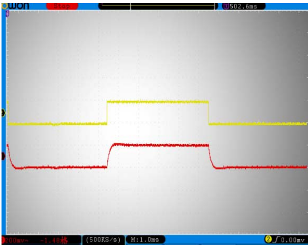
Figure 14 Small Signal Modulation
