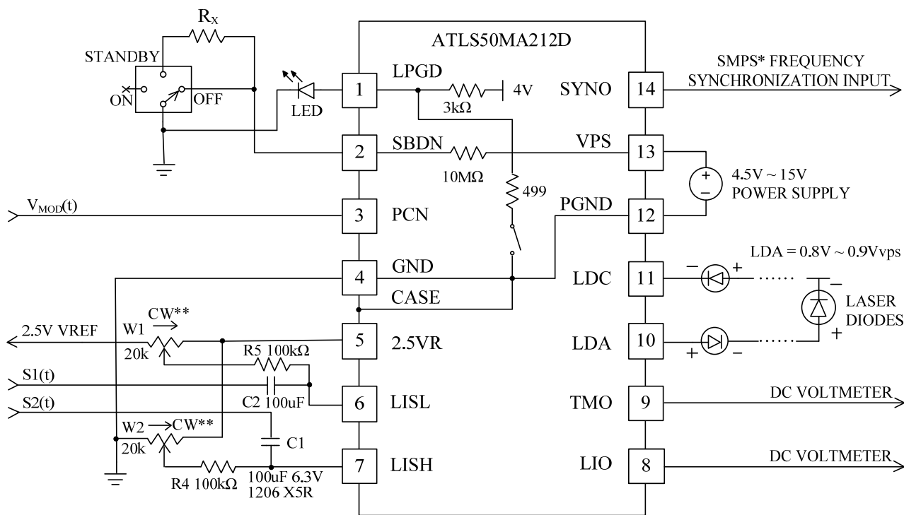
Figure 8. Digitally Controlled Analog Modulation Principle
