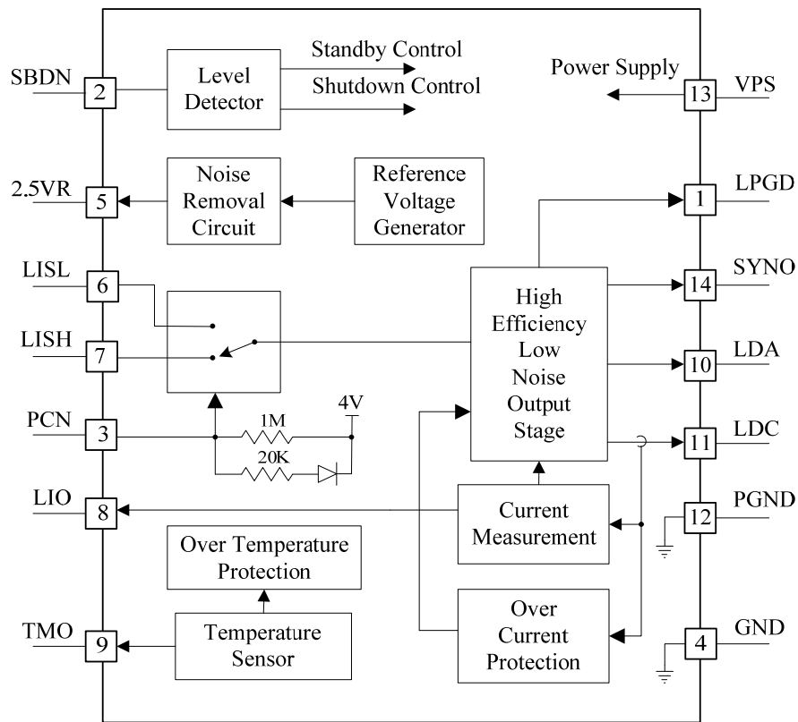
Figure 3. Internal Block Diagram of ATLS50MA212
