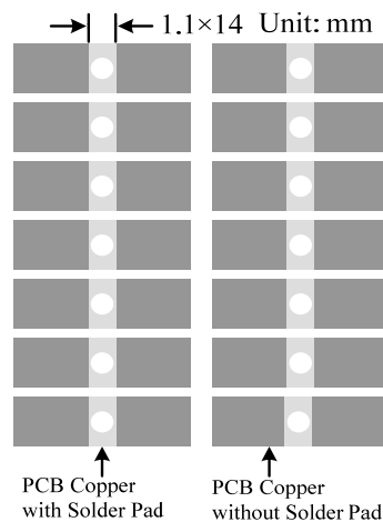
Figure 18. Top View of the Bottom Side PCB Foot-print
