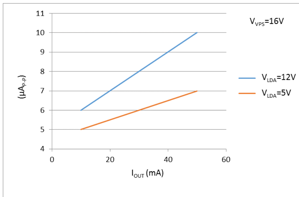
Figure 12.2. I_{OUT} vs. Output Current Noise@0.1Hz~10Hz
