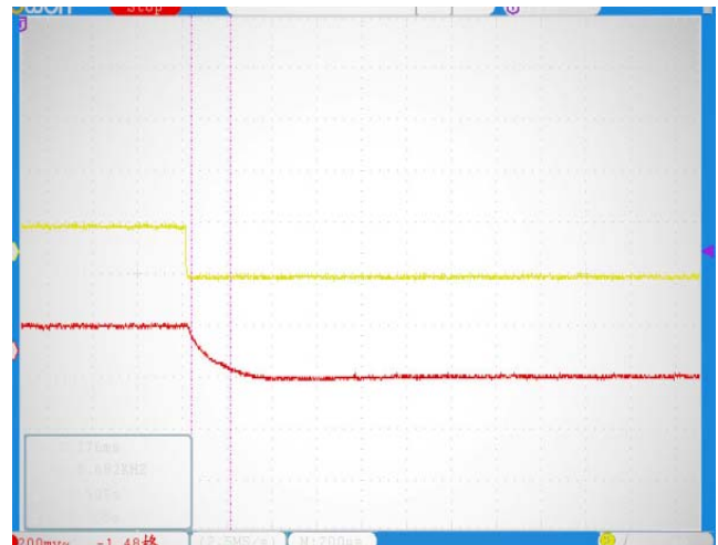
Figure 14.2. The Fall Signal Modulation
