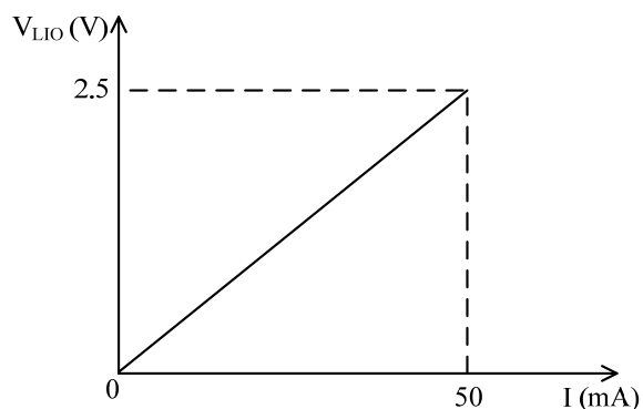
Figure 6. Using V_{LIO} to read the output current.
