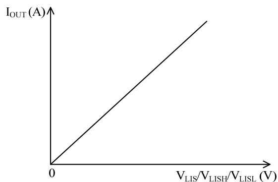
Figure 5. Using V_{LISH} and V_{LISL} to set the output current.
