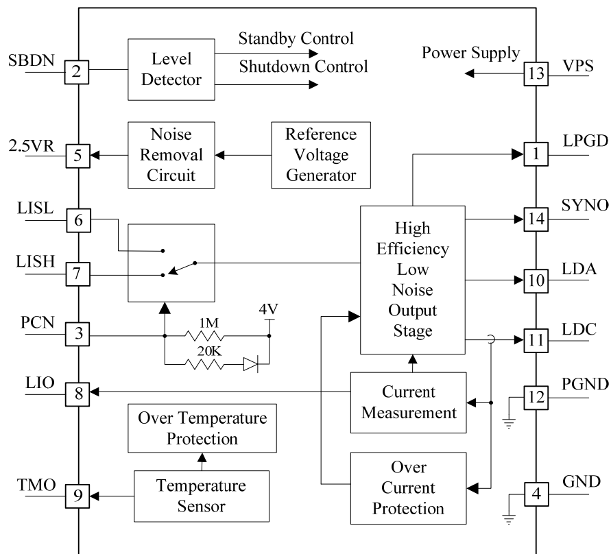
Figure 3. Internal Block Diagram of ATLS500MA212
