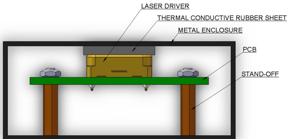
Figure 9.1 Transferring Heat with Metal Enclosure
