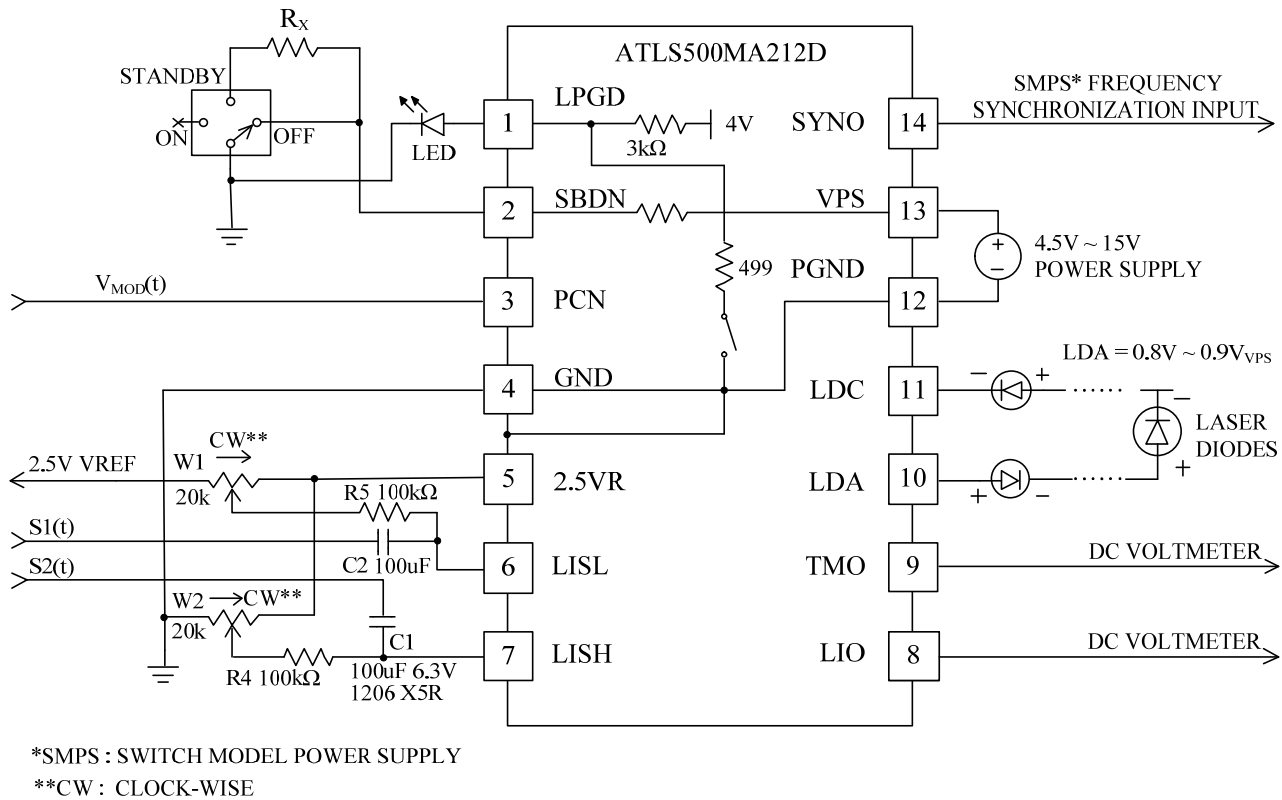
Figure 7. A Typical Stand-alone Application Schematic
