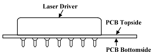
Figure 15. Side View of the Laser Driver mounted on PCB
