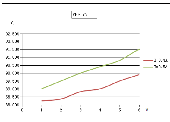
Figure 12. The efficiency of the laser driver.
