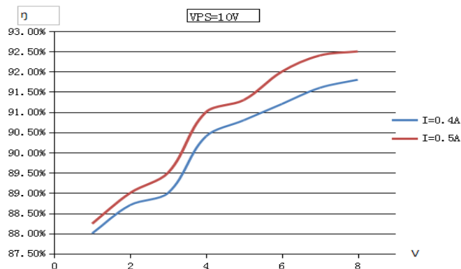
Figure 12. The efficiency of the laser driver.
