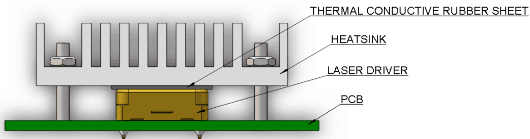
Figure 9.2 Transferring Heat with Heat Sink
