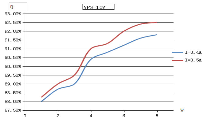
Figure 12. The efficiency of the laser driver.
