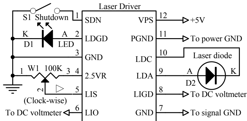
Figure 4.1. A Typical Stand-alone Application Schematic for ATLS500MA201D
