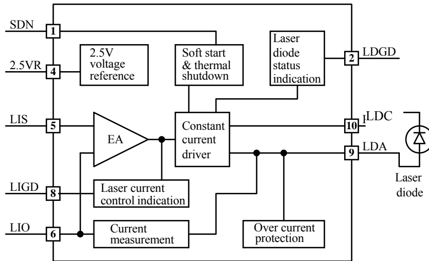
Figure 3. Block Diagram
