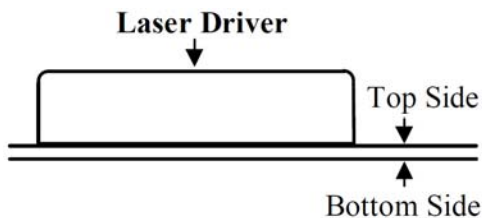
Figure 12. End View of the PCB Foot-print
