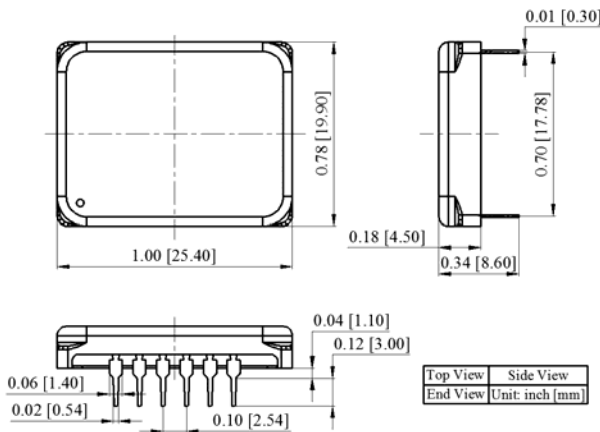
Figure 11. Dimensions of the DIP Package Driver Laser Driver
