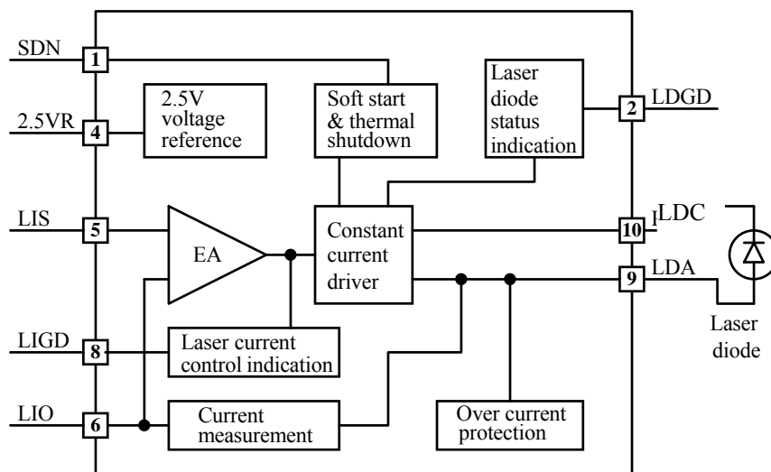
Figure 3. Block Diagram
