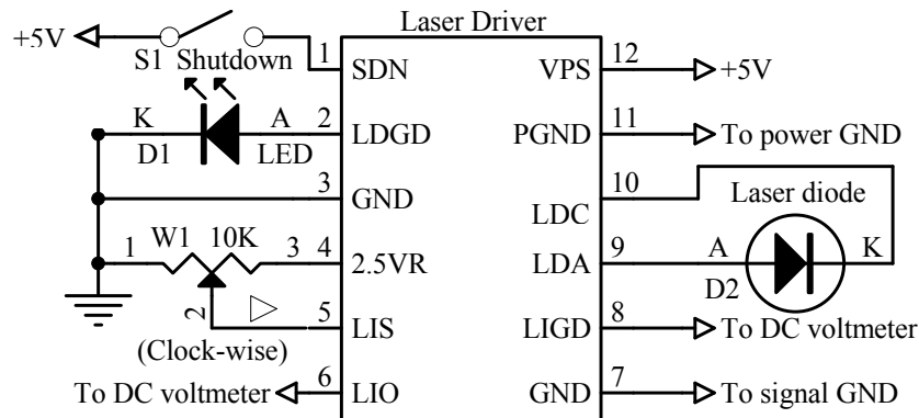
Figure 4.2. A Typical Stand-alone Application Schematic for ATLS500MA201D-PD
