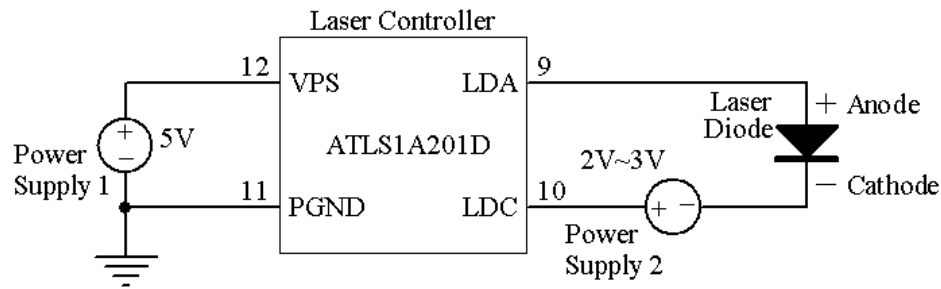
Figure 8. Driving High Voltage Laser Diodes
