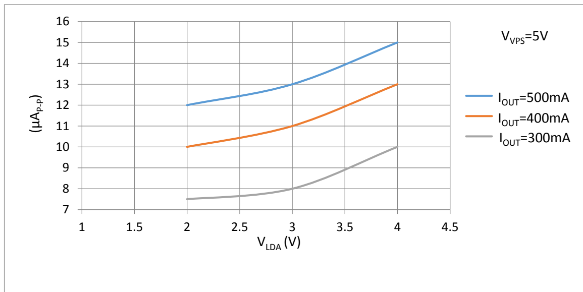
Figure 10. V LDA vs. Output Current Noise@0.1Hz~10Hz
