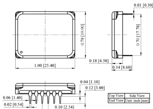
Figure 11. Dimensions of the DIP Package Driver
