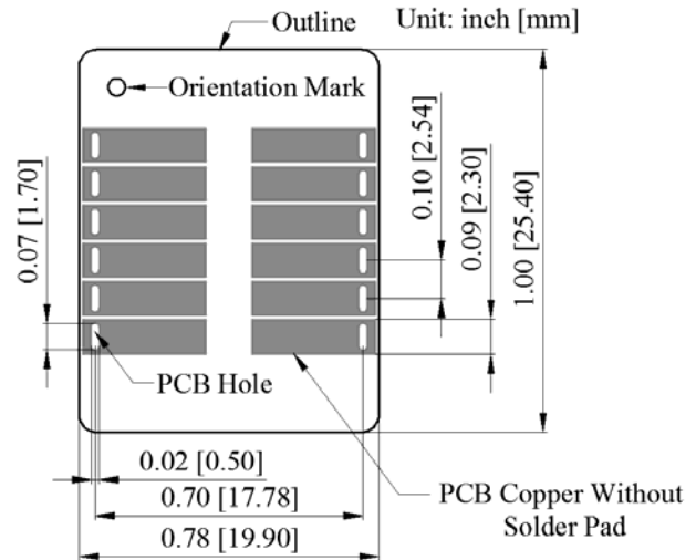
Figure 13. Top View of the Top Side PCB Foot-print
