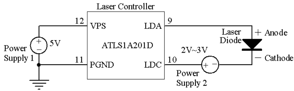
Figure 8. Driving High Voltage Laser Diodes
