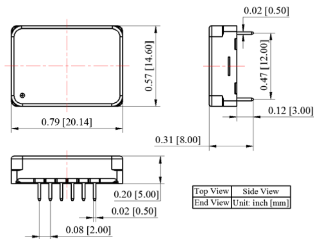
Figure 21. Dimensions of the DIP Package Controller
