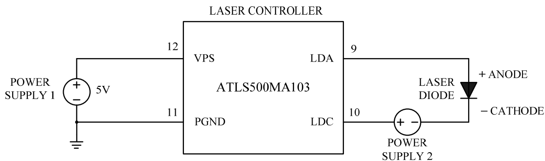
Figure 19. Driving High Voltage Laser Diodes
