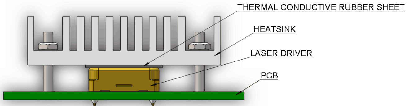
Figure 15.1 Transferring Heat with Heat Sink
