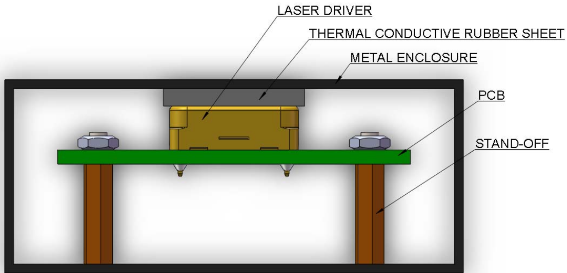
Figure 15.2 Transferring Heat with Metal Enclosure
