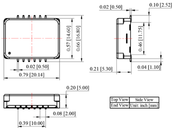
Figure 22. Dimensions of the SMT Package Controller
