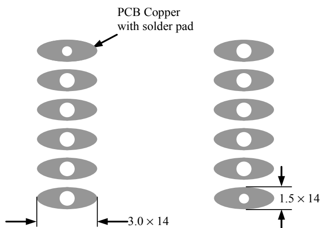
Figure 23. Top Side PCB Foot-print for the DIP Package
