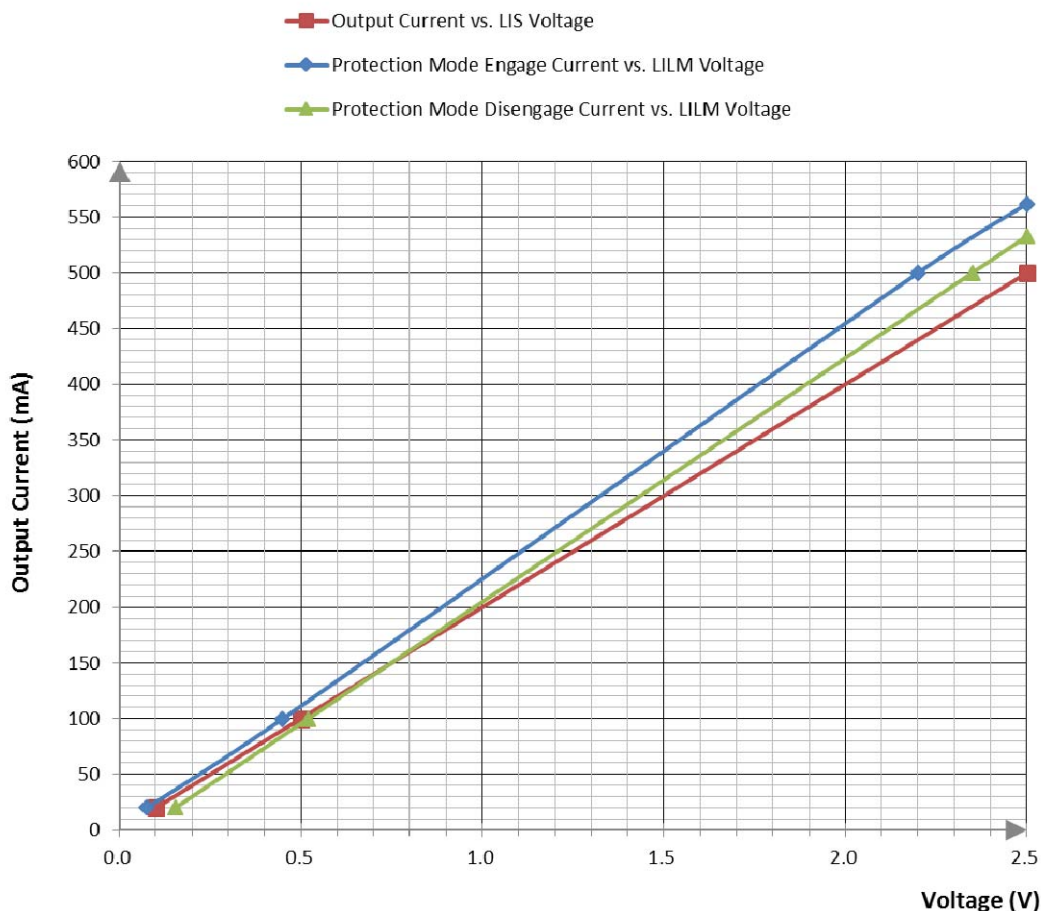
Figure 20. Output Current vs. LIS and LILM Voltage
