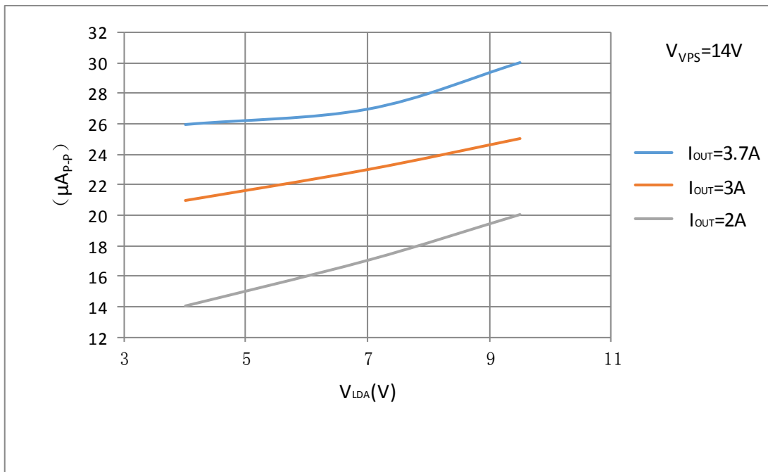
Figure 9.1. V_{LDA} vs. Output Current Noise@0.1Hz~10Hz
