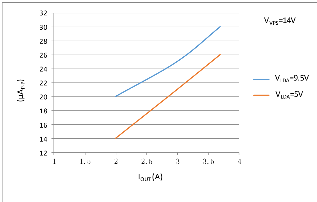
Figure 9.2. I_{OUT} vs. Output Current Noise@0.1Hz~10Hz
