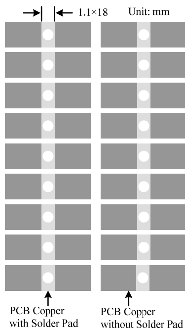
Figure 15. Top View of the Top Side PCB Foot-print
