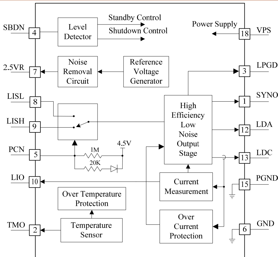
Figure 3. Internal Block Diagram of ATLS4A214
