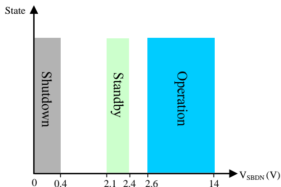
Figure 4. Input Control
