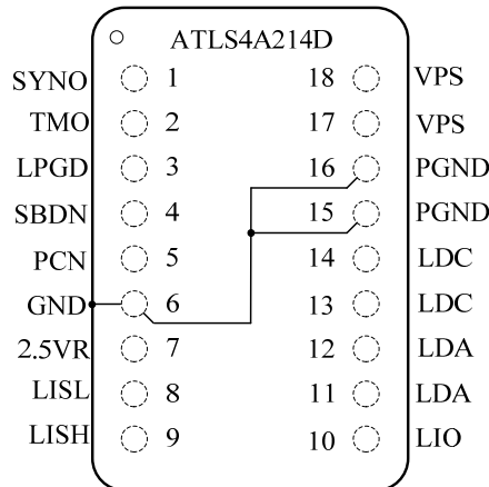
Figure 2. Pin Names and Locations
