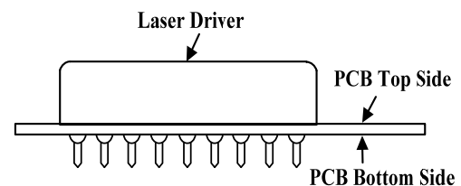
Figure 14. End View of the PCB Foot-print
