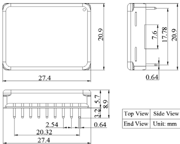
Figure 12. Dimensions of the DIP Package Driver
