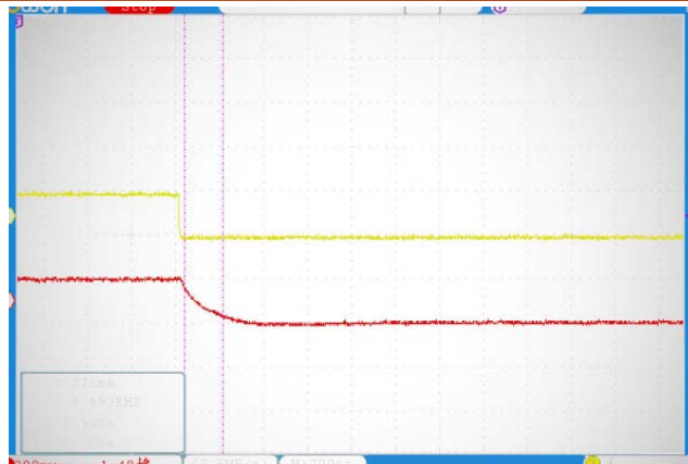
Figure 11.3. The Fall Signal Modulation
