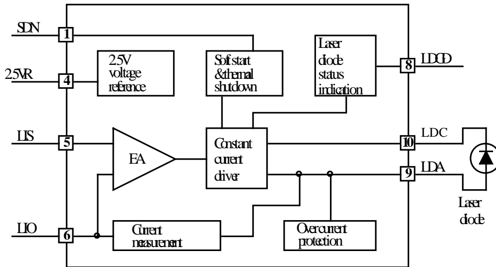
Figure 3. Block Diagram
