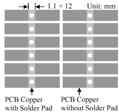
Figure 10. Top View of the Bottom Side PCB Foot-print Figure 10 shows the top view of the bottom side PCB foot-print.
