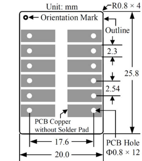
Figure 9. Top View of the PCB Foot-print
