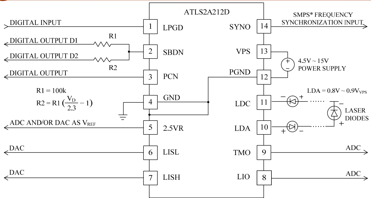
Figure 8. A Typical Micro-processor-based Application Schematic
