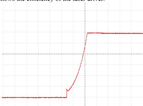
The soft start of startup by both power supply and the switch. When the current is 0.2A, the voltage is 6V.
