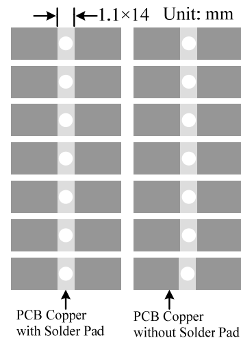
Figure 17. Top View of the Bottom Side PCB Foot-print
