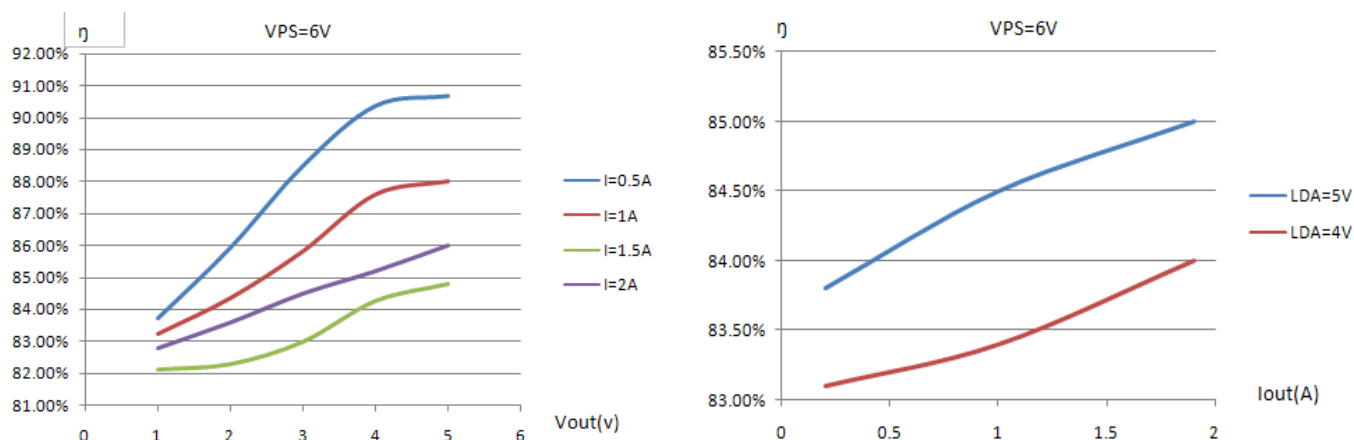
Figure 12. Efficiency of Laser Driver
