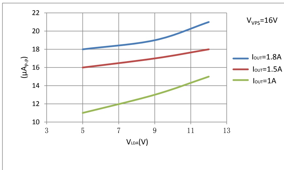
Figure 10.2. I_{\text{OUT}} vs. Output Current Noise@0.1Hz~10Hz
