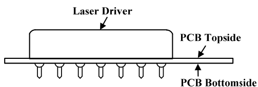
Figure 15. End View of the PCB Foot-print
