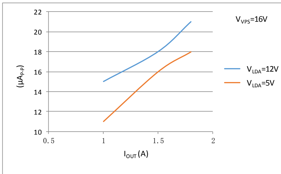
Figure 10.1. V_{\text{LDA}} vs. Output Current Noise@0.1Hz~10Hz
