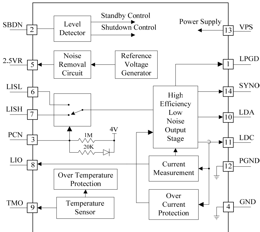
Figure 3. Internal Block Diagram of ATLS2A212
