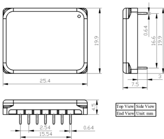
Figure 14. Dimensions of the DIP Package Driver
