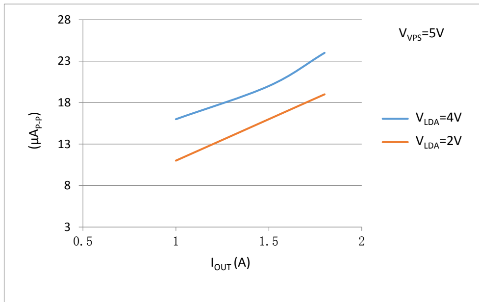
Figure 10. I_{\text{OUT}} vs. Output Current Noise@0.1Hz~10Hz
