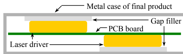
Figure 8. Transferring heat by the gap filler
