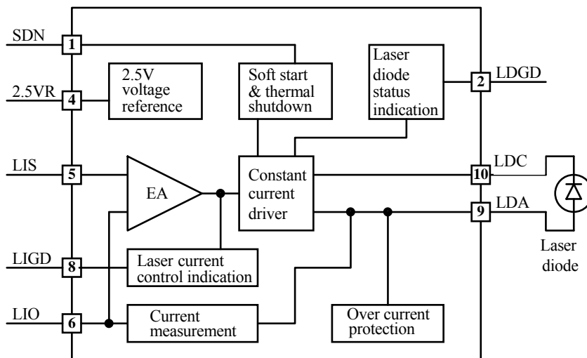
Figure 3. Block Diagram
