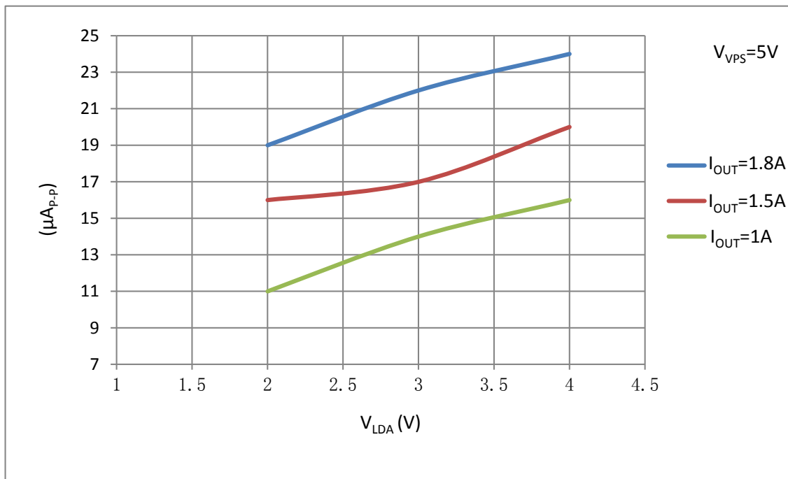
Figure 9. V_{\text{LDA}} vs. Output Current Noise@0.1Hz~10Hz
