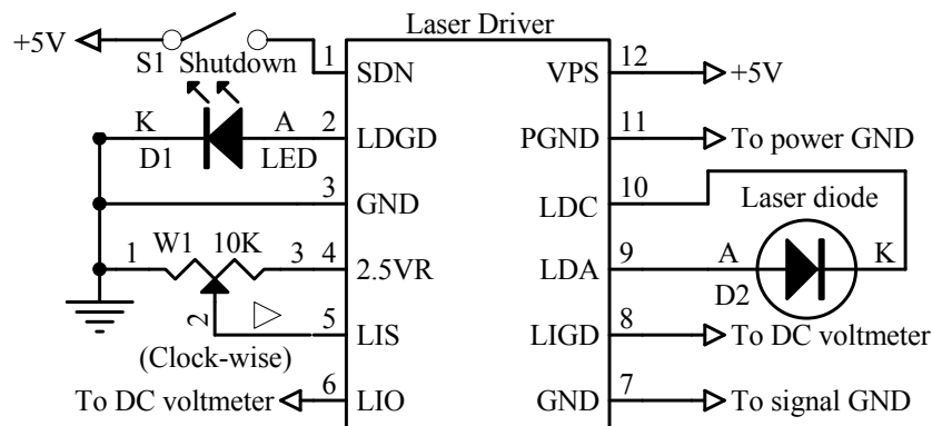
Figure 4.2. A Typical Stand-alone Application Schematic for ATLS2A201D-PD
