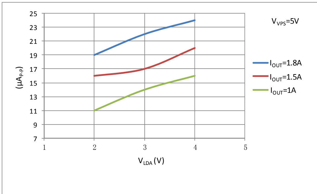
Figure 9. V_{LDA} vs. Output Current Noise@0.1Hz~10Hz
