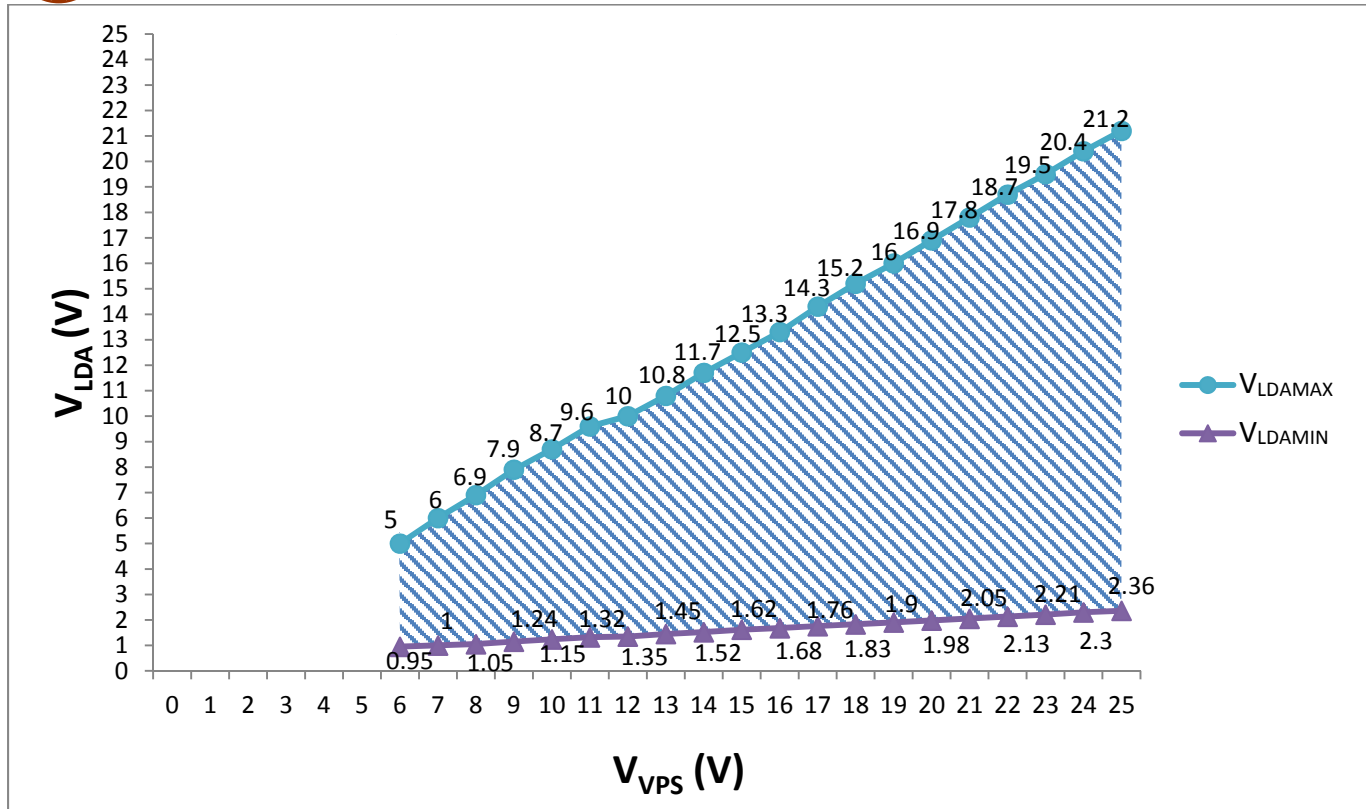
Figure 15. V VPS vs. V LDA
