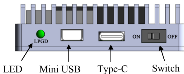
Figure 3. Side View
