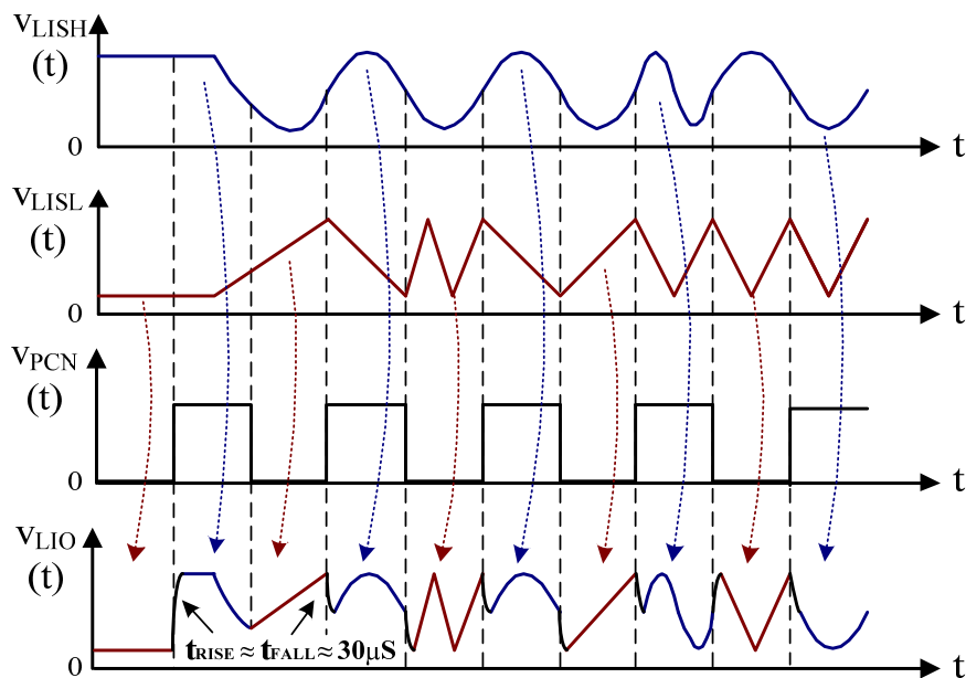
Figure 12. Digitally Controlled Analog Modulation Principle
