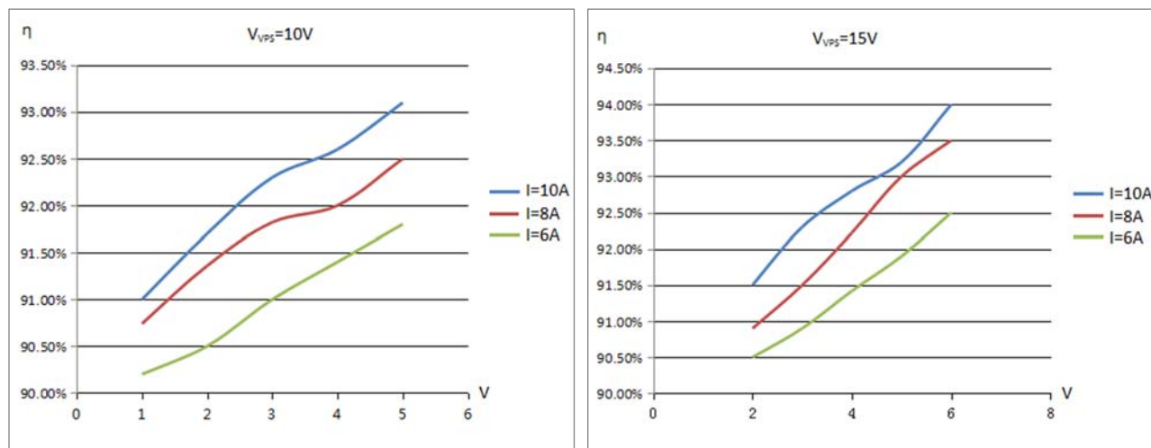
Figure 9. Efficiency of Laser Driver
