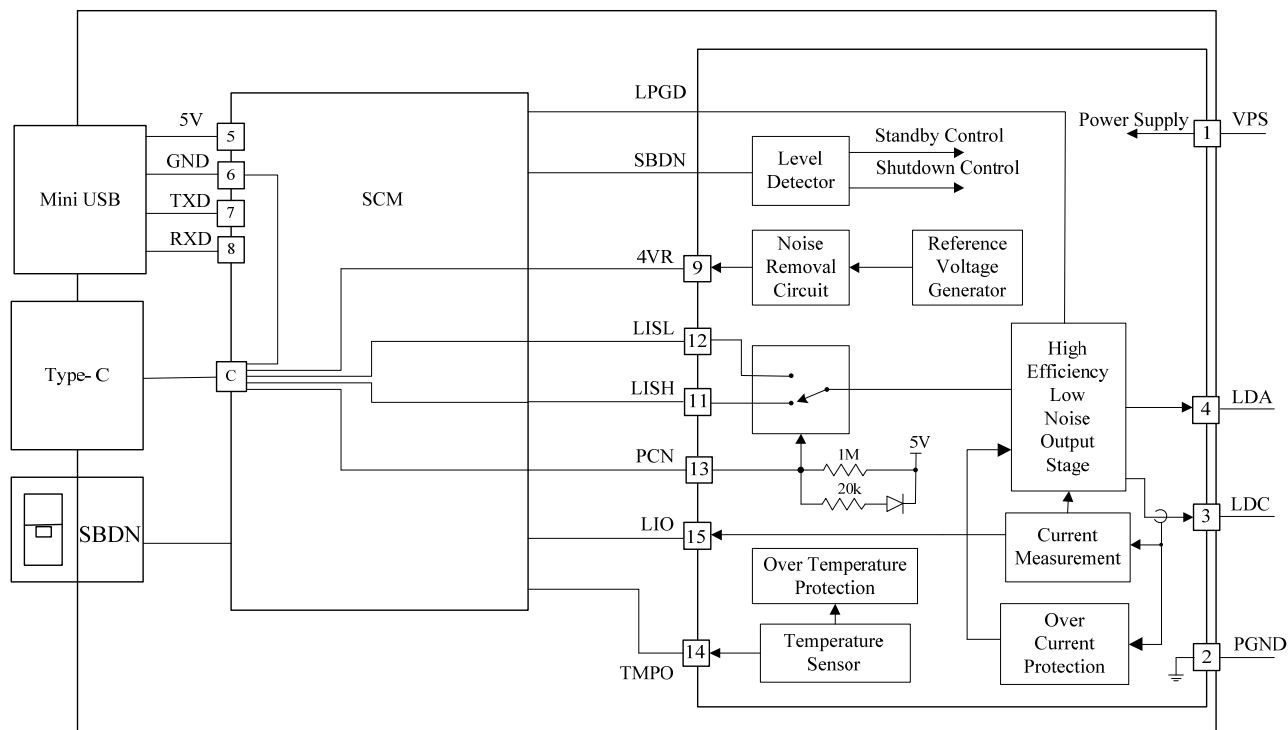
Figure 6. Internal Block Diagram of ATLS25A219GUI
