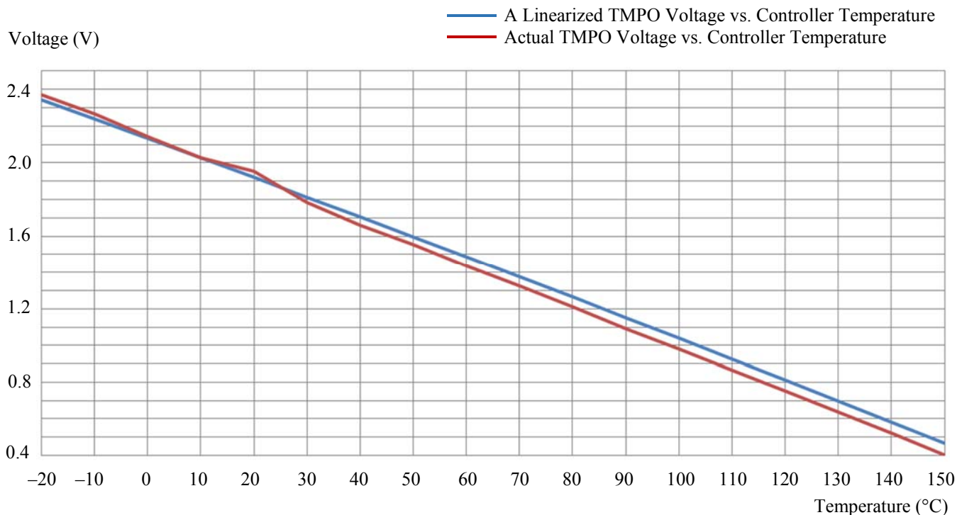
Figure 8. Controller Internal Temperature vs. TMPO Voltage
