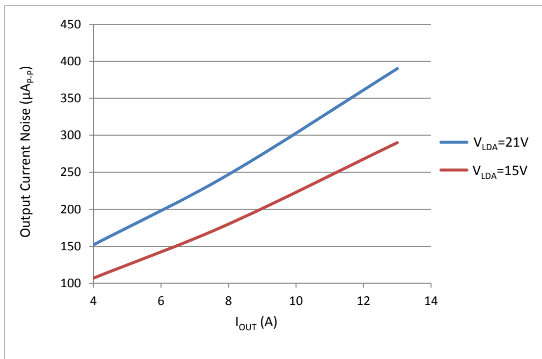
Figure 14. I_{\text{OUT}} vs. Output Current Noise@0.1Hz~10Hz
