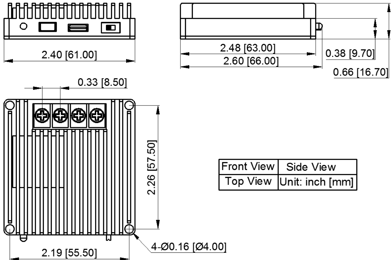
Figure 17. Dimensions of ATLS25A219GUI
