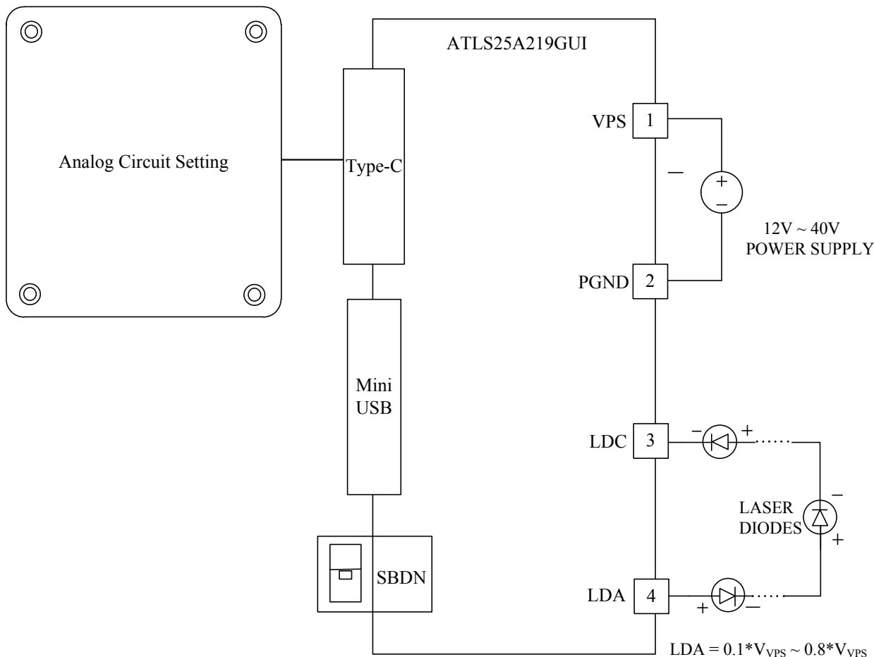
Figure 11. Micro-Controller Based Application Schematic
