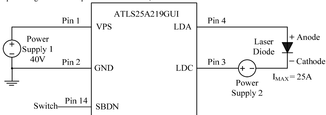
Figure 16. Driving High Voltage Laser Diodes
