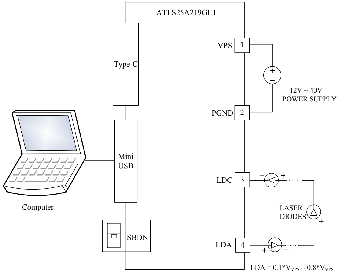
Figure 10. Stand-Alone Application Schematic
