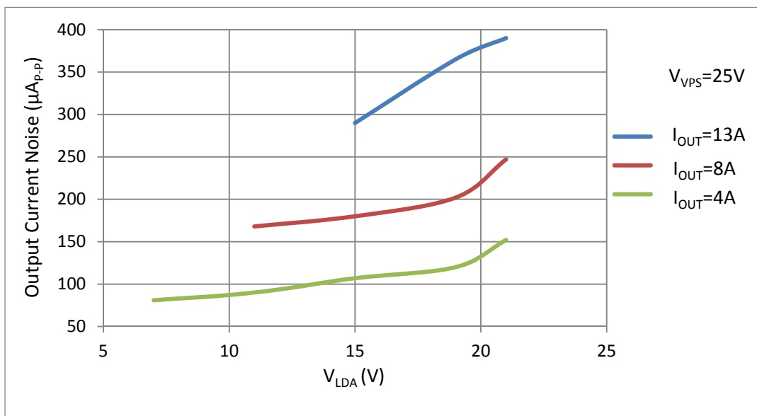
Figure 13. V_{\text{LDA}} vs. Output Current Noise@0.1Hz~10Hz
