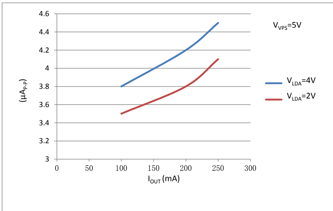
Figure 10. 2. I_{OUT} vs. Output Current Noise@0.1Hz~10Hz
