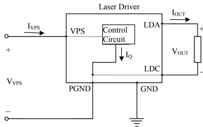
Figure 7. The Current Distributions in the Controller
