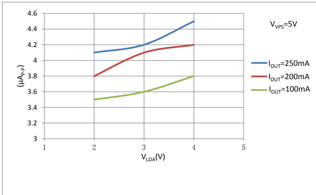
Figure 10. 1. V_{LDA} vs. Output Current Noise@0.1Hz~10Hz
