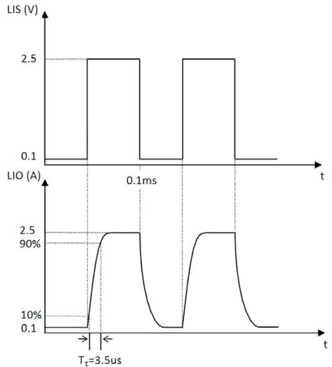
Figure 9. Large Signal Modulation
