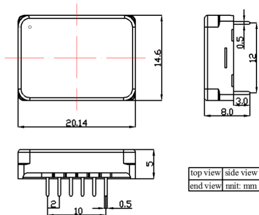
Figure 11. Dimensions of the DIP Package Controller
