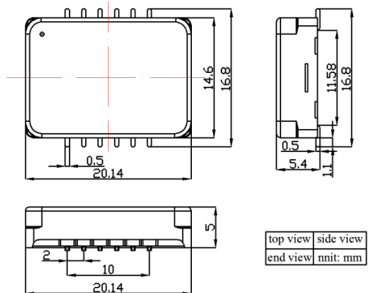
Figure 12. Dimensions of the SMT Package Controller
