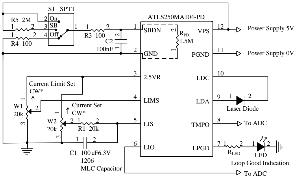
Figure 5.2. Typical Stand-alone CW Operation Schematic for ATLS250MA104-PD
