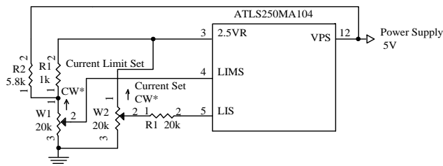
Figure 7. V_{LIMS} setting larger than V_{LIS}
