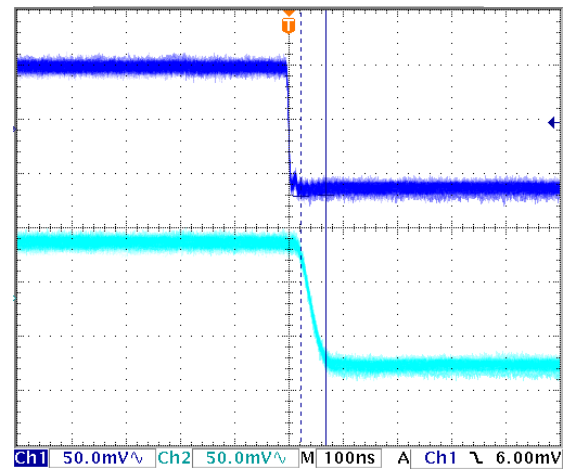
Figure 12.4. Small Signal Fall Time 46ns
