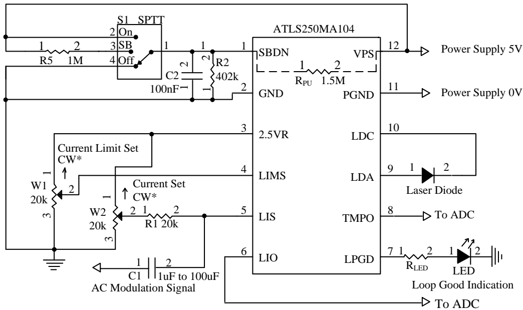
Figure 5.3. Typical AC Modulation with DC bias Schematic for ATLS250MA104
