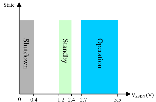
Figure 3. Input Control
