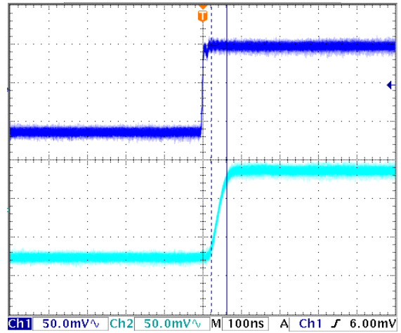
Figure 12.3. Small Signal Rise Time 40ns
