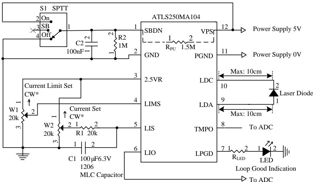
Figure 5.1. Typical Stand-alone CW Operation Schematic for ATLS250MA104
