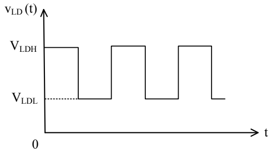
Figure 9.2. Laser Diode Voltage v_{LD}(t) Waveform
