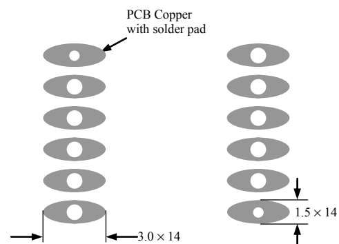
Figure 23. Top View of the Bottom Side PCB Foot-print
