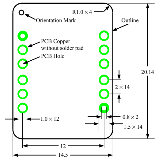
Figure 22. Top Side PCB Foot-print for the DIP Package
