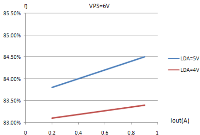
Figure12. Efficiency of Laser Driver
