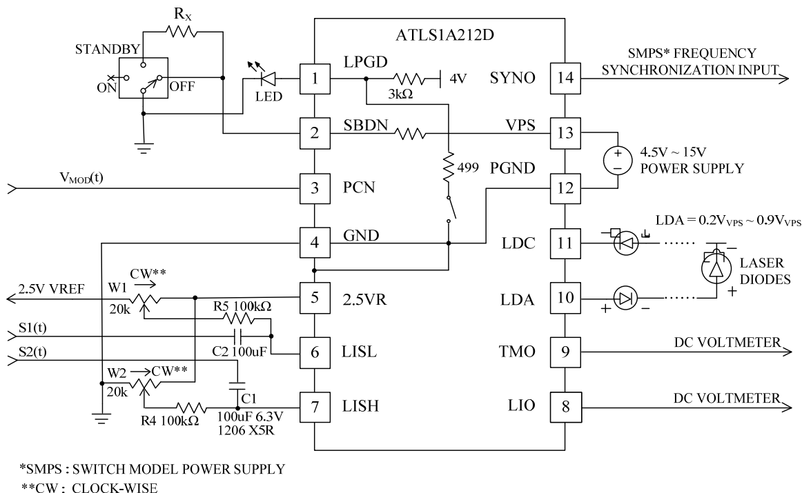
Figure 6. A Typical Stand-alone Application Schematic
