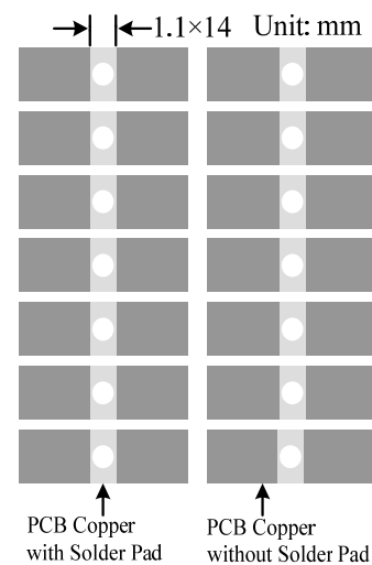
Figure 17. Top View of the Bottom Side PCB Foot-print Figure 17 shows the foot-print which is seen from the bottom side of the PCB.
