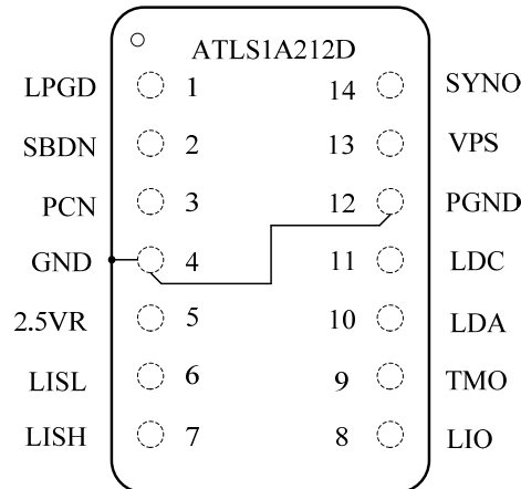
Figure 2. Pin Names and Locations
