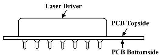
Figure 15. End View of the PCB Foot-print
