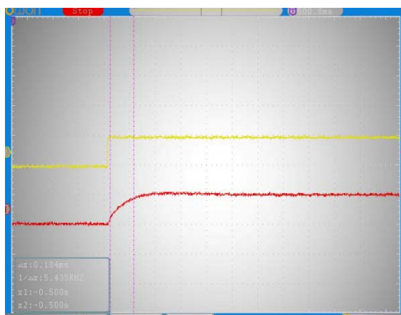
Figure 13.1. The Rise Signal Modulation
