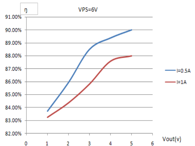
Figure12. Efficiency of Laser Driver
