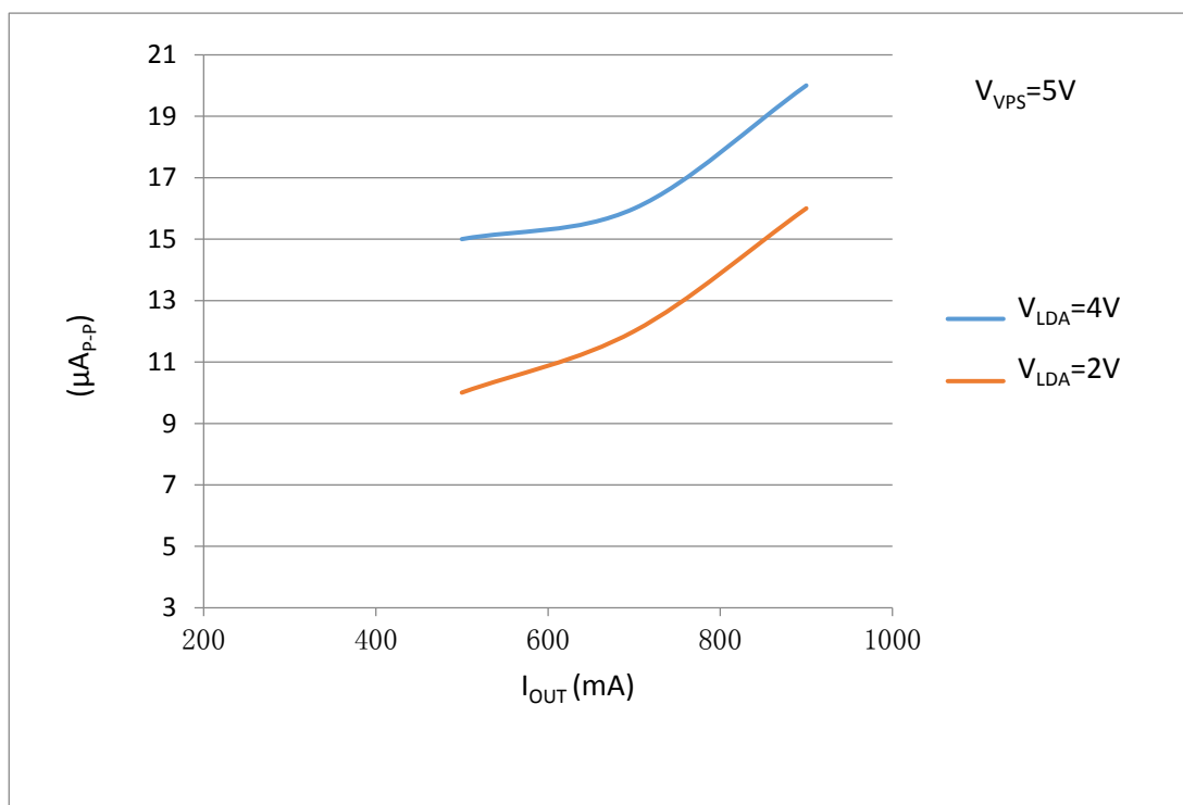
Figure 7. 2. I_{\text{OUT}} vs. Output Current Noise@0.1Hz~10Hz
