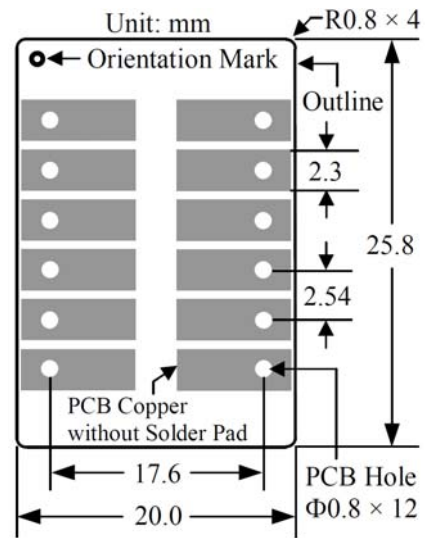
Figure 9. Top View of the PCB Foot-print
