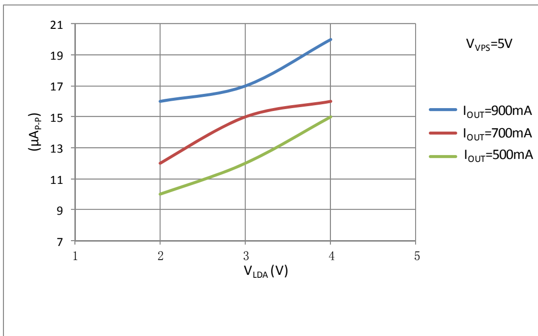
Figure 7. 1. V_{\text{LDA}} vs. Output Current Noise@0.1Hz~10Hz
