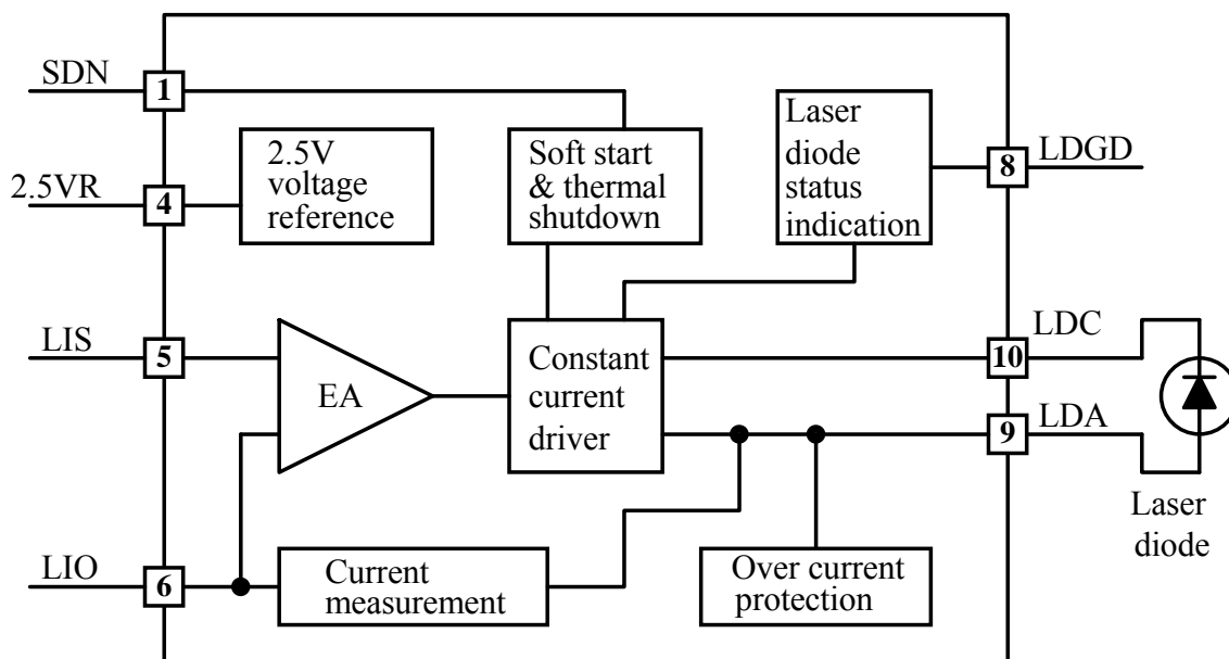
Figure 3. Block Diagram
