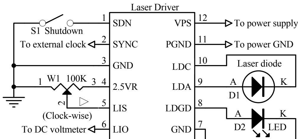
Figure 4. A Typical Stand-alone Application Schematic
