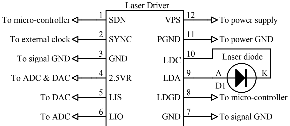
Figure 5. A Typical Micro-processor-based Application Schematic
